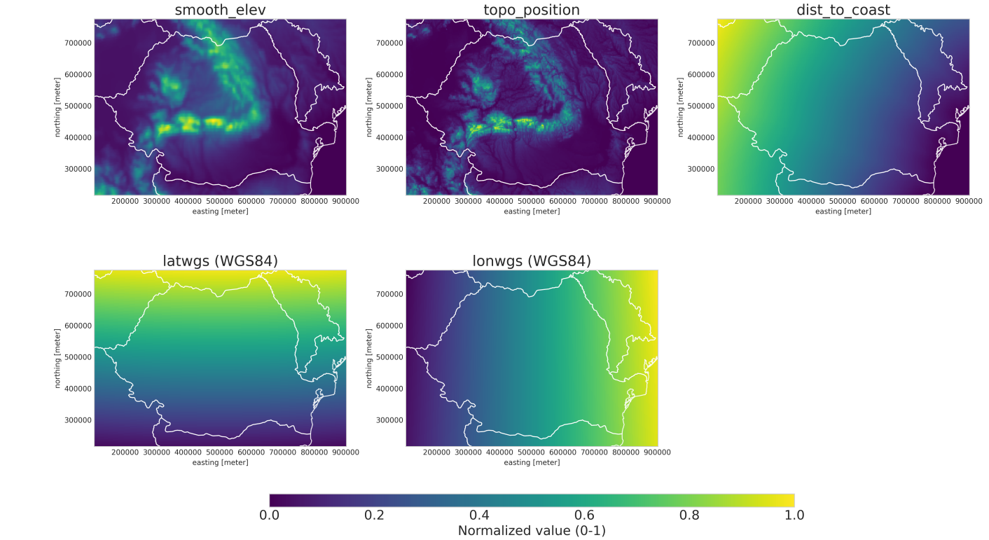
Figure 2 Static predictors derived from DEM.
