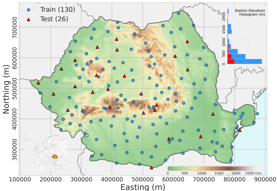
110 Figure 1 Spatial distribution of the 156 meteorological stations used in this study, overlaid on the SRTM digital elevation model of Romania. Training stations ( n = 130 , blue circles) and held-out test stations ( n = 26 , red triangles) were assigned by random spatial split. The inset histogram shows the elevation distribution of training and test stations, confirming that both subsets span the full altitudinal range of the network (0–2,544 m). Coordinates are in the Dealul Piscului 1970 projection (EPSG:31700). Inset map shows Romania’s location within Europe. SRTM data © NASA / NGA.
