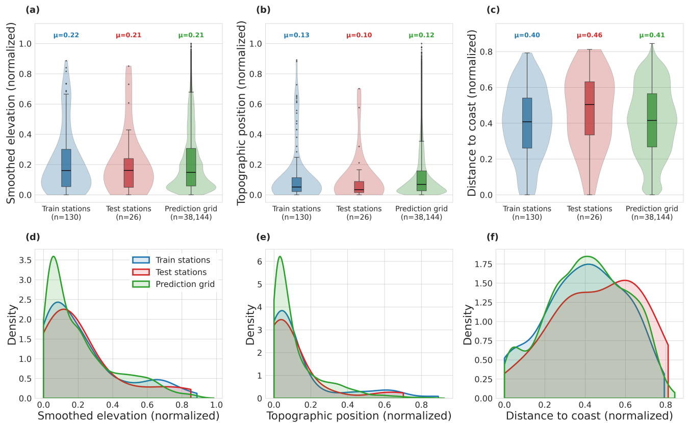
145 Figure 3 Distribution of key static predictors across training stations ( n = 130 ), test stations ( n = 26 ), and prediction grid cells within Romania ( n = 38,144 ). (a–c) Violin plots with overlaid box plots for smoothed elevation, topographic position index, and distance to the Black Sea coast, respectively; the mean value ( \mu ) for each distribution is indicated at the top of the panels. (d–f) Kernel density estimates for the same three predictors. Predictor values are shown in their normalized [0, 1] form.
