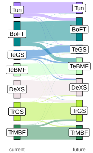
(c) RCP85
