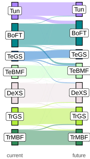
(a) RCP26
