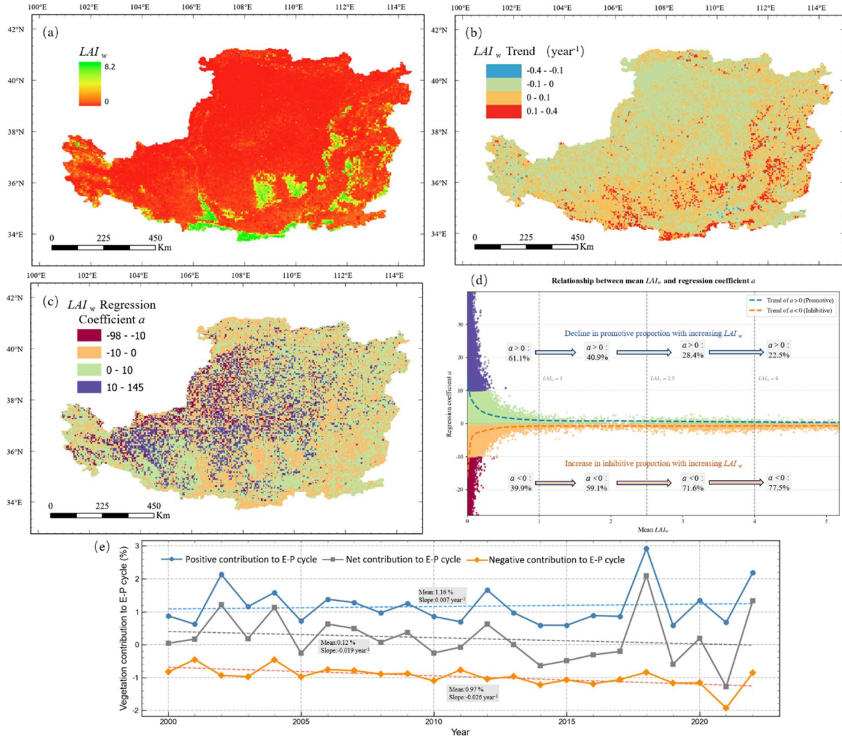
350 Figure 4. Spatial patterns and effects of vegetation-weighted index LAI_w over the Loess Plateau. (a) Spatial distribution of mean LAI_w during the growing season. (b) Spatial patterns of linear trends in LAI_w . (c) Spatial distribution of the regression coefficient a . (d) Relationship between mean LAI_w and the regression coefficient a . (e) Interannual variation of vegetation contributions to the evaporation–precipitation cycle.
