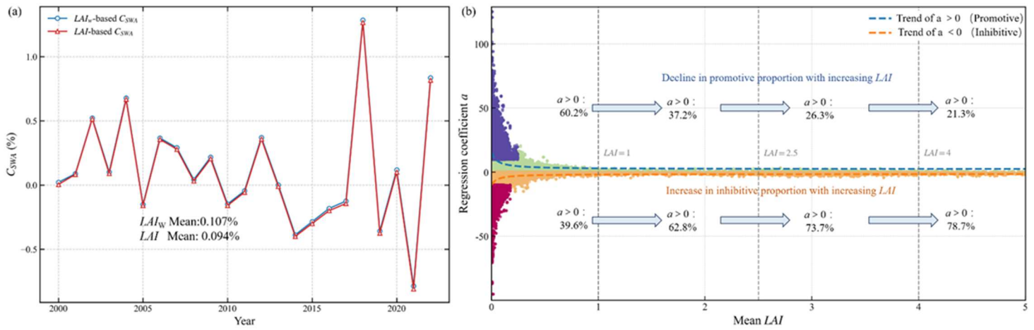
530 Figure 7: Vegetation-associated related variations in surface water availability and vegetation contribution under LAI and LAI_w conditions: (a) interannual variations in vegetation-associated related C_{SWA} estimated from LAI and LAI_w , (b) contribution rates of vegetation to SWA under promotive and inhibitive conditions along the mean LAI gradient.
