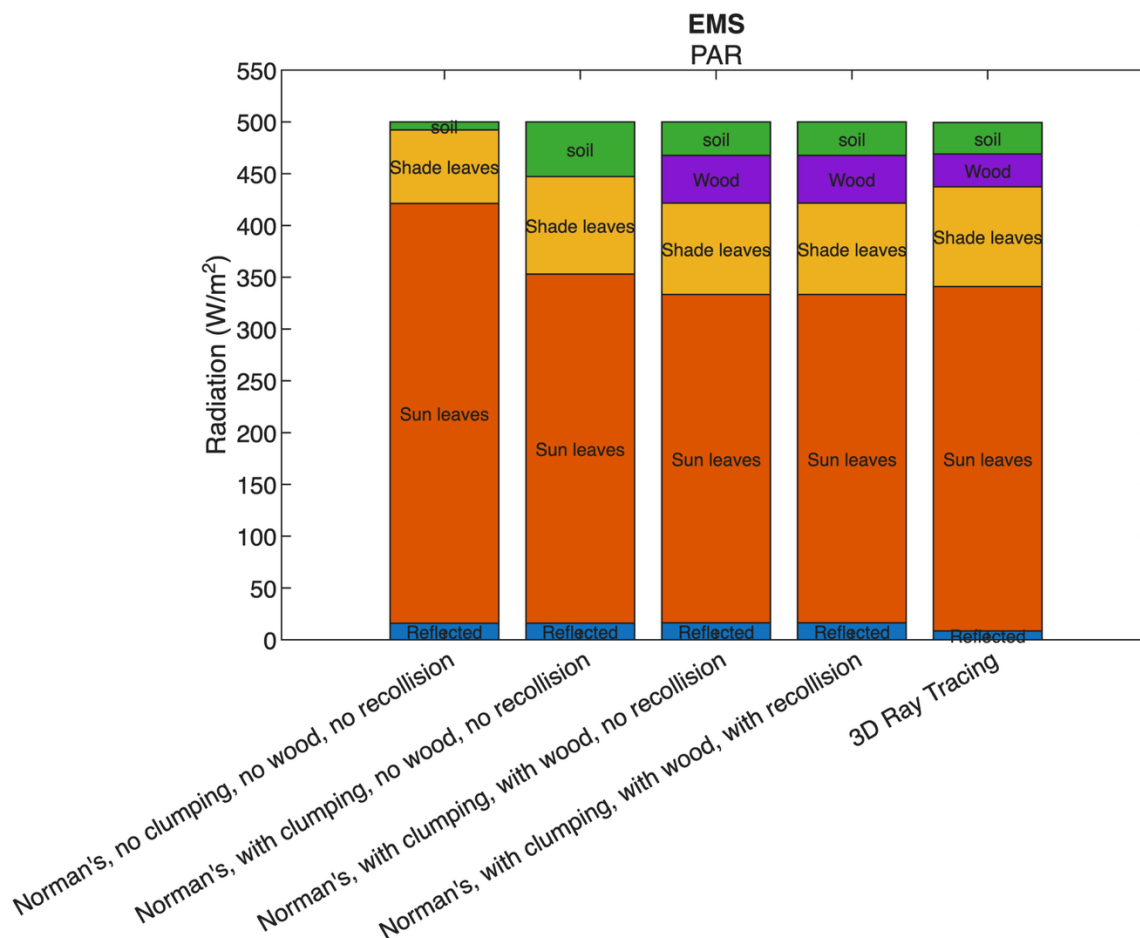
360 Figure 2: Budget for the proportions of NIR (top) and PAR (bottom) reflected, and absorbed by sunlit and shaded leaves, by wood and soil, simulated using the Norman model with four different configurations and the FLiESvox 3D ray tracing model. All simulations are for sun zenith angle of 35 degrees, diffuse fraction of 20% and incoming radiation of 500 W/m 2 . Shown here are results for the Harvard Forest site (equivalent figures for all other sites are provided in Supporting Information)
