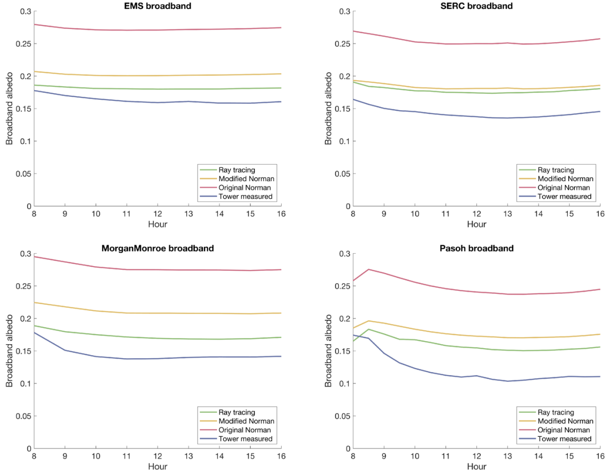
Figure 5: Tower observed and modeled using the modified Norman (in yellow), Norman model version presented in Béland and Baldocchi (2021) (here labeled Original Norman, in red), and FLiESvox (in green) models for shortwave albedo at all sites. Diurnal patterns are averages for each hour at Harvard Forest and Morgan Monroe, and half hour at SERC and Pasoh, for the month of July at all sites except Pasoh which is for February.
