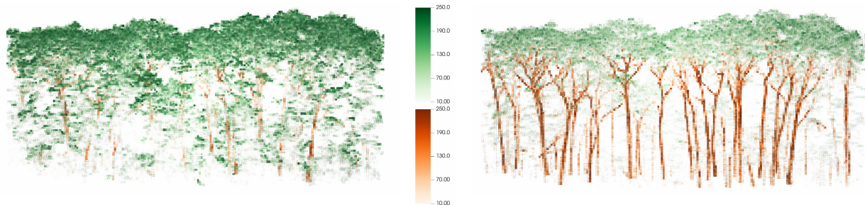
Figure 1: Examples of a 3D voxel-based mapping of absorbed radiation (in Watts per m 2 ) by leaves (green) and wood (brown) in PAR (left) and NIR (right) as simulated by the FLiESvox 3D raytracing radiative transfer model at the Harvard Forest site.
