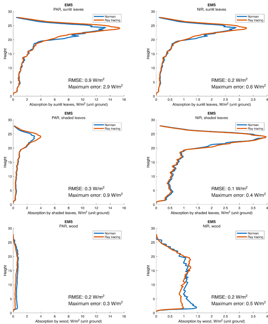
395 Figure 4: Vertical profiles of absorbed radiation by sunlit leaves (top), shaded leaves (middle), and wood (bottom) in the PAR (left) and NIR (right) for Norman (blue lines) and FLiESvox (red lines) models. Data shown here is for the Harvard Forest site, data for all sites is provided in Supporting Information.
