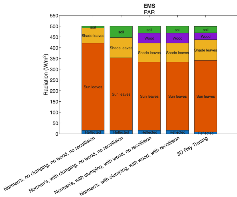
365 Figure 2: Budget for the proportions of NIR (top) and PAR (bottom) reflected, and absorbed by sunlit and shaded leaves, by wood and soil, simulated using the Norman model with four different configurations and the FLiESvox 3D ray tracing model. All simulations are for sun zenith angle of 35 degrees, diffuse fraction of 20% and incoming radiation of 500 W/m 2 . Shown here are results for the Harvard Forest site (equivalent figures for all other sites are provided in Supporting Information)
