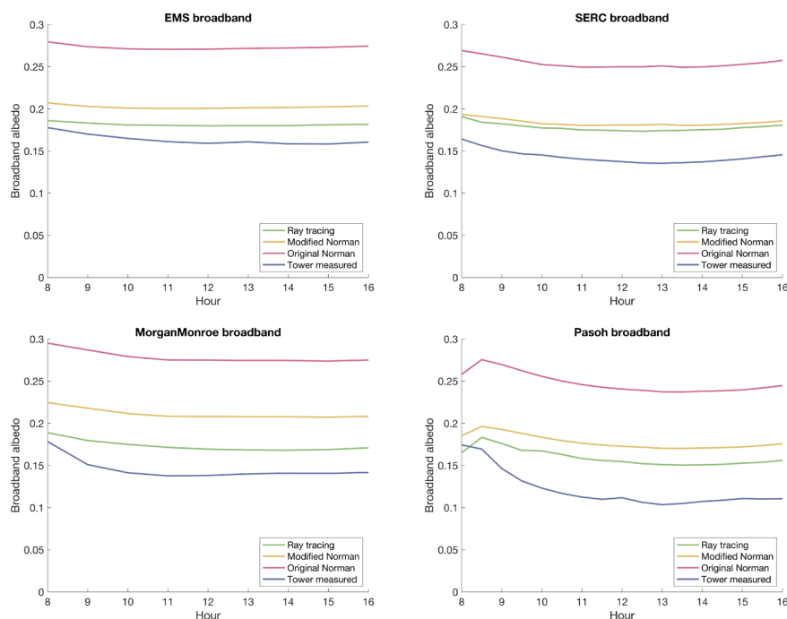
Figure 5: Tower observed and modeled using the modified Norman (in yellow), Norman model version presented in B eland and Baldocchi (2021) (here labeled Original Norman, in red), and FLiESvox (in green) models for shortwave albedo at all sites. Diurnal patterns are averages for each hour at Harvard Forest and Morgan Monroe, and half hour at SERC and Pasoh, for the month of July at all sites except Pasoh which is for February.
