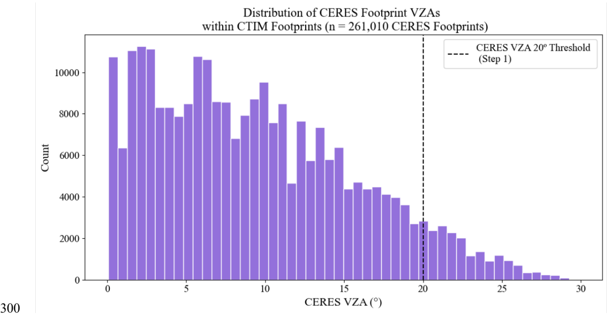
Figure 8: Distribution of CERES VZAs within CTIM footprints. The black line exhibits the VZA 20^\circ threshold applied in Step 1 of the matching algorithm, showing the 6.93% of CERES footprints with a VZA greater than 20^\circ resulting from Step 2.
