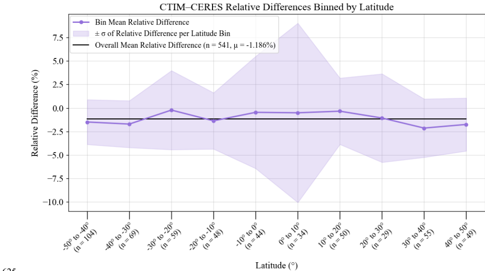
Figure 17: Mean CTIM–CERES relative difference and \pm 1\sigma envelope binned by 10° latitude intervals for all 541 matches. The mean relative difference remains close to the overall mean of -1.19% across most latitude bins with no clear latitudinal trend. The two largest spreads occur in the -10° to 0° ( n = 44 , \sigma = 5.97\% ) and 0° to 10° ( n = 34 , \sigma = 9.54\% ) latitude bins, compared to all other bins ( \sigma = 2.38 -4.71%), consistent with the persistent deep convective cloud cover and enhanced scene heterogeneity of the ITCZ.
