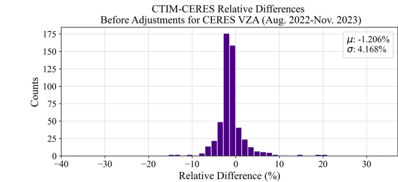
Figure 11: Distribution of relative differences (see Eq. (7)) between CTIM and CERES before applying adjustments for CERES VZA. CERES radiances were only weighted by the CTIM response function.
