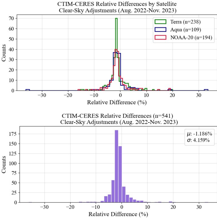
710 Figure 14: Relative difference histograms between CTIM and CERES measured longwave radiances for 541 matches. Top: Relative differences between CTIM and CERES radiance measurements for Terra, Aqua, and NOAA-20. Bottom: Relative differences between CTIM and CERES, where CERES represents the collective data from CERES aboard Terra, Aqua, and NOAA-20.
