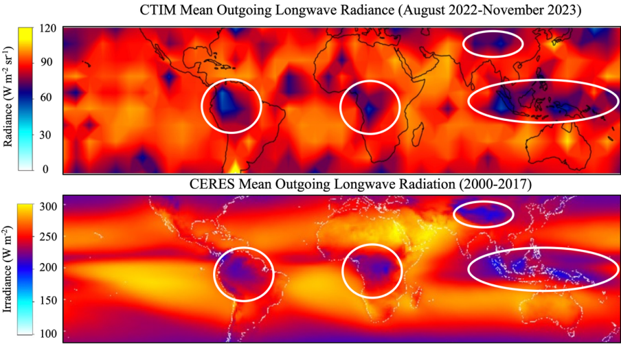
295 Figure 7: Global longwave radiation. Top: All CTIM longwave radiance from the A1 detector during orbital eclipse (nighttime observations) spatially gridded at \sim 4^\circ resolution for 15 months of observations. All observed radiances within an approximate 4^\circ bin were bin-averaged to determine the pixel radiance within the CTIM latitude range. Bottom: CERES all-sky outgoing longwave radiation ( daytime and nighttime ) averaged over seventeen years of observations from Terra and Aqua (adapted from Dewitte and Clerbaux, 2018). Yellow-red regions represent areas of high longwave radiation emission, and purple-blue regions represent areas of low longwave radiation emission. Note the CERES radiative energy is expressed in irradiance ( \text{W m}^{-2} ), and the CTIM radiative energy is expressed in radiance ( \text{W m}^{-2} \text{sr}^{-1} ). A direct quantitative comparison between the two is not straightforward, as converting radiance to irradiance requires assumptions about the angular distribution of emitted radiation that do not hold uniformly across all scene types. Despite the different units, localized concentrations of radiative energy are qualitatively similar, specifically low areas of radiative energy that are highlighted by the white circles.
