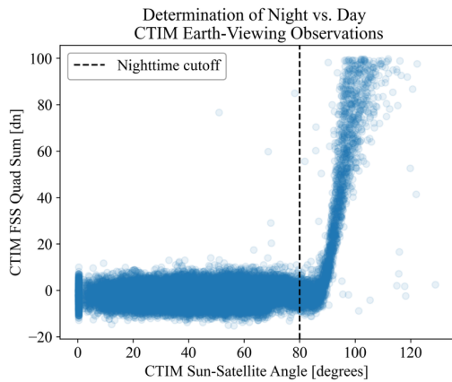
265 Figure 4: Determination of CTIM Earth-eclipsed observations from the CTIM FSS Quad Sum and CTIM Sun-Satellite Angle. Datapoints accepted as eclipsed data had a Sun-satellite angle less than 80° .
