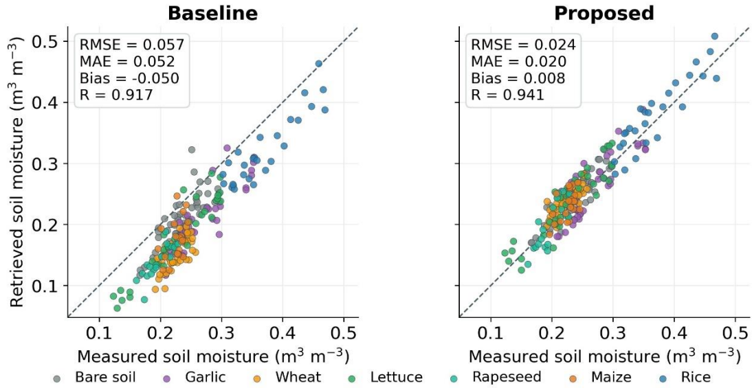
Figure 5. Retrieved versus observed surface soil moisture for the baseline inversion and the proposed Bayesian joint retrieval. The 1:1 line indicates unbiased retrieval, and points represent matched validation observations grouped by land-cover class.
