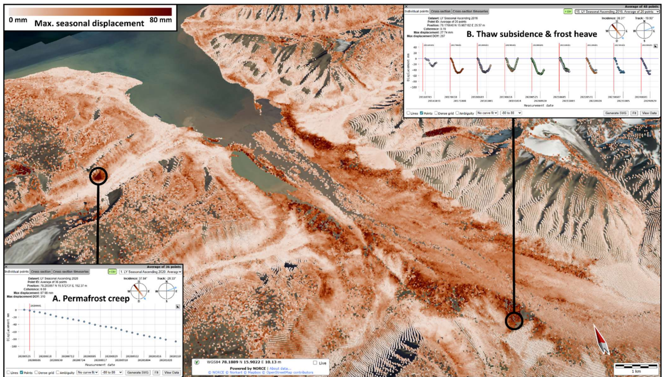
135 Figure 2. Example of seasonal InSAR Svalbard results in the Longyearbyen (LY) study area. The map displays the maximum seasonal displacement expressed in mm (here for 2020, using an ascending SAR geometry). A. When analysing one SAR geometry and one season, the seasonal time series provide information on the short-term displacement pattern during the spring–fall snow-free period (here on a rock glacier). B. When all seasons and geometries are viewed all together, the time series provide information about the magnitude and timing of the displacement patterns during multiple seasons (here cyclic 140 subsidence–heave patterns in an ice-rich part of the Advent valley). The results are shown in the InSAR Svalbard WebGIS tool. Background: Svalbard Orthophoto (NPI, 2026).
