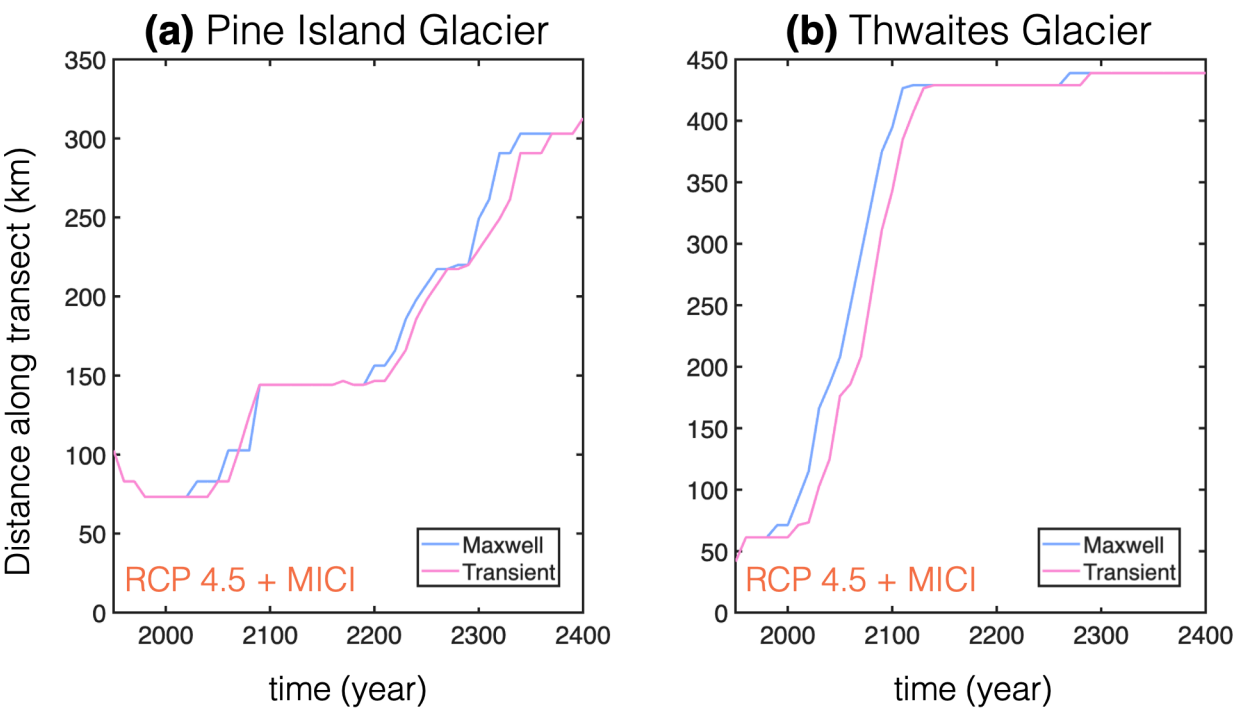
Figure S16. Grounding line migration including MICI (a),(b) Timeseries of Maxwell and transient model grounding line position along transects for Pine Island (a) and Thwaites glacier under RCP 4.5, including the MICI (corresponds to Figure 7 from the Main Text).
