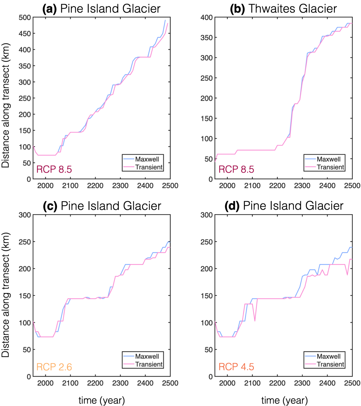
Figure S15. Grounding line migration (a),(b) Timeseries of Maxwell and transient model grounding line position along transect for Pine Island (a) and Thwaites glacier (b) under RCP 8.5 (corresponds to Figure 3 from the Main Text). (c),(d) Timeseries of Maxwell and transient model grounding line position along Pine Island transect for Pine Island under RCP 2.6 (c) and RCP 4.5 (d), corresponding to Figure 4 from the Main Text.
