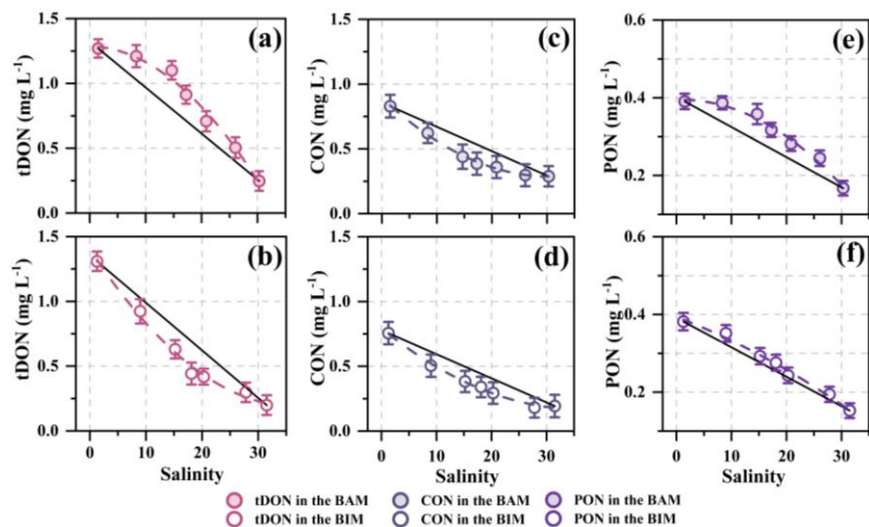
205 Figure 1. Variations in the concentrations of truly dissolved organic nitrogen (tDON) (a, b), colloidal organic nitrogen (CON) (c, d) and particulate organic nitrogen (PON) (e, f) across different river-seawater mixing ratios in the biologically active mixing (BAM) and biologically inhibited mixing (i.e., physicochemical mixing only, BIM) treatments. Conservative mixing curves (solid lines) were calculated using a two-end-member model based on the river-water and seawater endmembers (Langmuir et al., 1978), while dashed lines represent smoothed fits to the observed data. Deviations of the observed data from the conservative mixing curves indicate non-conservative behavior, with positive deviations representing net addition and negative deviations representing net removal.
