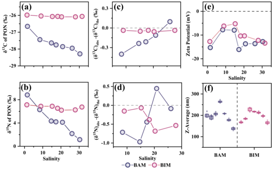
Figure 34. Variations of \delta^{13}\text{C} values of particulate organic nitrogen (PON) (a), \delta^{15}\text{N} values of PON (b), zeta potential (e), and mean particle size (f) along the salinity gradient in the biologically active mixing (BAM) and biologically inhibited mixing (i.e., physicochemical mixing only, BIM) treatments. Panels c and d show the deviations of \delta^{13}\text{C} and \delta^{15}\text{N} values of PON, respectively, calculated as the difference between the observed values ("obs") under mixed salinity conditions and the theoretical values ("the") predicted by the two-end-member model.
