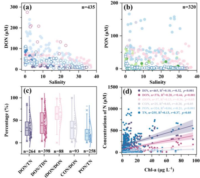
470 Figure 5. Non-conservative behavior of dissolved organic nitrogen (DON) (a) and particulate organic nitrogen (PON) (b) along the salinity gradient in estuarine mixing zones of rivers discharging into the global ocean. Different colors and symbols (hollow and solid) represent different estuaries; detailed site information is provided in Table S4S6 . (c) Boxplots showing the proportions of DON and PON relative to total nitrogen (TN), DON relative to total dissolved nitrogen (TDN), and the distribution of truly dissolved organic nitrogen (tDON) and colloidal organic nitrogen (CON) within DON. (d) 475 Correlation analysis between organic nitrogen species and chlorophyll-a (Chl-a) concentrations in the water column.
