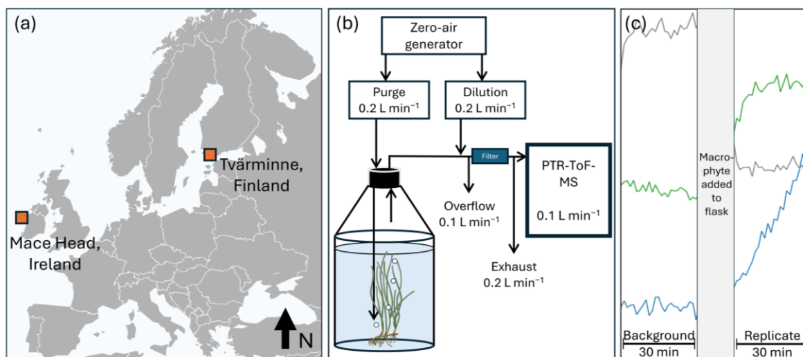
Figure 1: (a) Locations of the two study sites in Europe. (b) Schematic of the incubation setup. (c) Example data of three compounds with differing responses (see Section 2.6 for details on interpretation) after macrophyte addition: green line = Emission that quickly stabilizes, blue line = Emission that keeps increasing, and grey line = Uptake. Macrophyte image from Integration and Application Network (IAN), University of Maryland Center for Environmental Science ( https://ian.umces.edu/ , accessed 28.9.2026).
