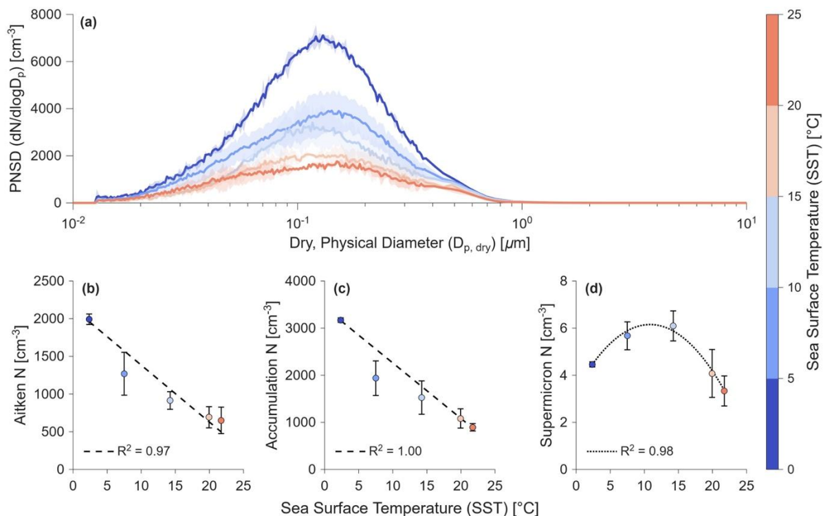
Figure 33: SST trends of SST-binned, and uncertainty-weighted PNSDs. (a) Mean PNSDs for five SST ranges measured by the SMPS-APS. Shaded regions indicate one standard deviation of the mean PNSD. (b) Total Aitken, (c) accumulation, and (d) supermicron mode number concentrations. The shaded regions in a and error bars in b-d indicate one standard deviation.
