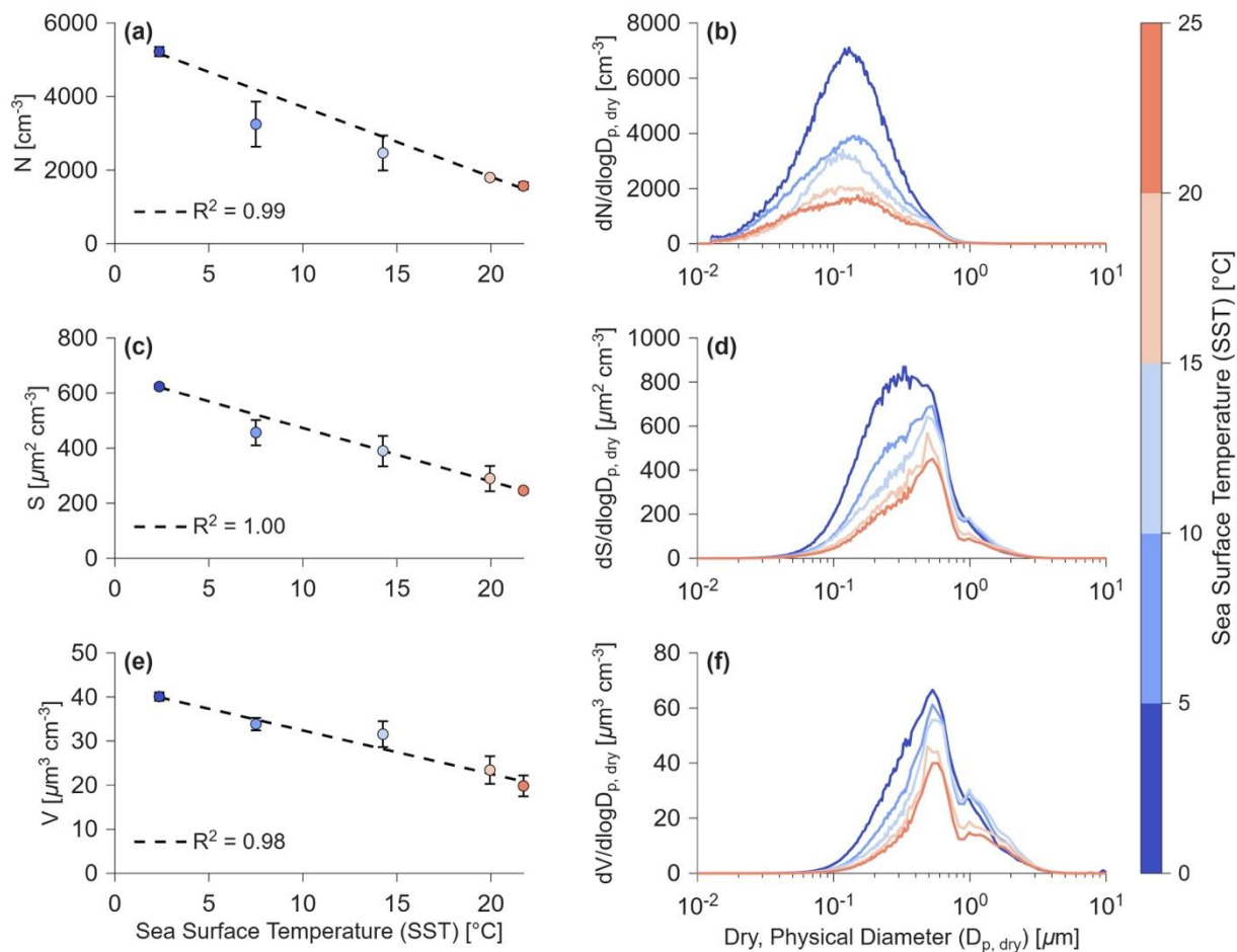
Figure 55: Higher order moments of the SST-binned, uncertainty-weighted PNSDs. (a) Total number, (c) surface area, and (e) volume of SSA in SOARS for each temperature range, with a dashed line representing a linear least squares best fit line. (b) Number, (d) surface area, and (f) volume size distribution for each temperature range.
