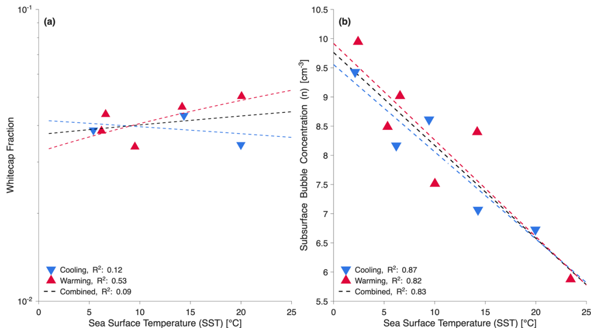
Figure 22: Trends in whitecap fraction and subsurface bubble concentrations. (a) Whitecap fraction and (b) subsurface bubble concentrations as a function of SST.
