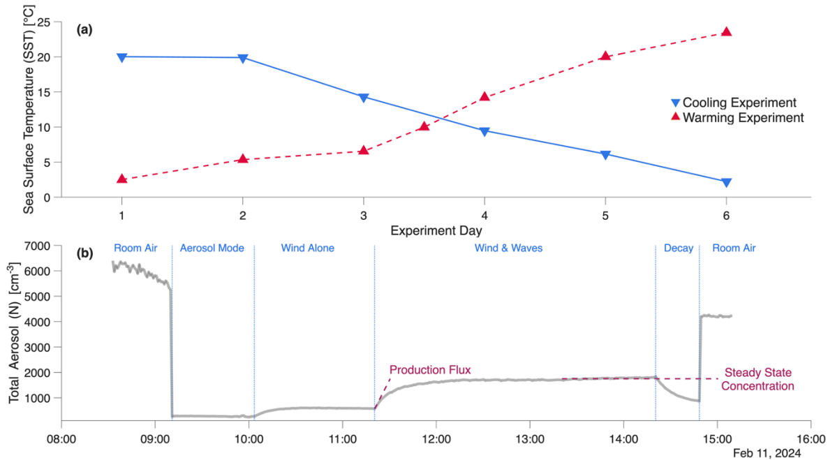
Figure 14: Experimental overview. (a) Sea surface temperature for each experimental day and (b) total aerosol number concentrations during a representative experimental day (11 February 2024, cooling experiment day 1), showing the size measurement periods of a daily experiment: Room Air, Aerosol Mode, Wind Alone, Wind & Waves, Decay. Magenta dashed lines indicate the Production Flux (concentration rise following wave onset) and Steady State Concentration (subsequent plateau), from which SSA number fluxes are derived (Sect. 3.5).
