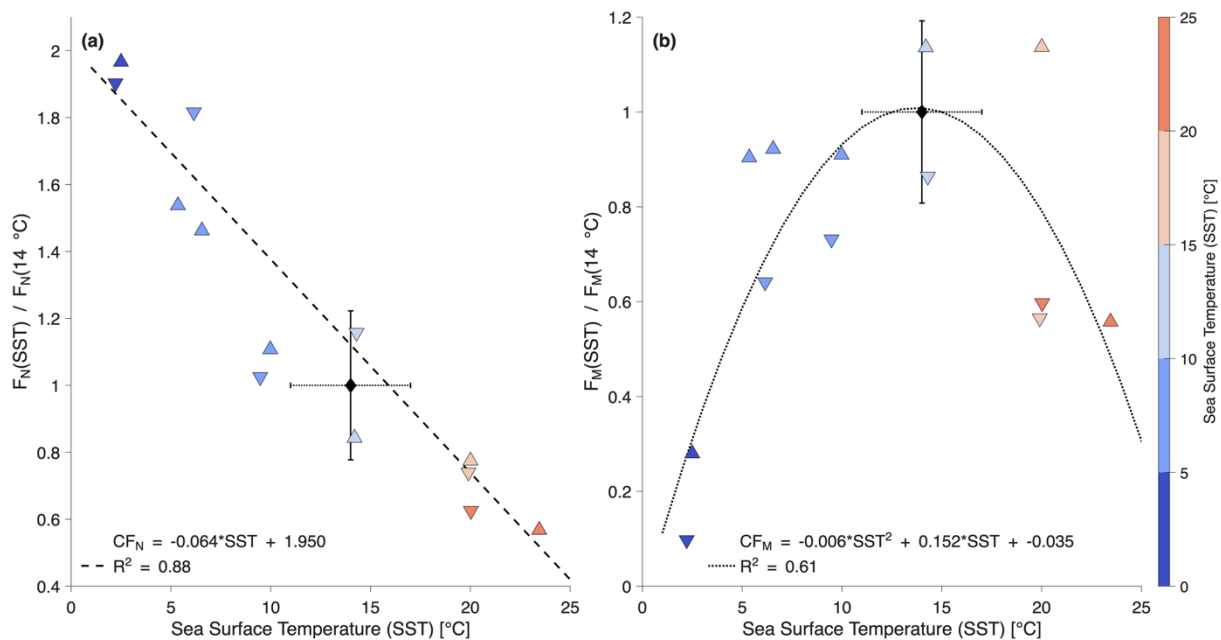
Figure 88: Correction factors applied to the complete sets of F_N and F_M measurements. (a) Total number emission flux ( F_N ) and (b) total mass emission flux ( F_M ) as a function of SST, normalized by the average flux at 14 °C. The black diamond depicts flux at 14 °C, and the vertical error bars represent one standard deviation. The horizontal error bars represent the annual SST range of the coastal seawater sourced for this study.
