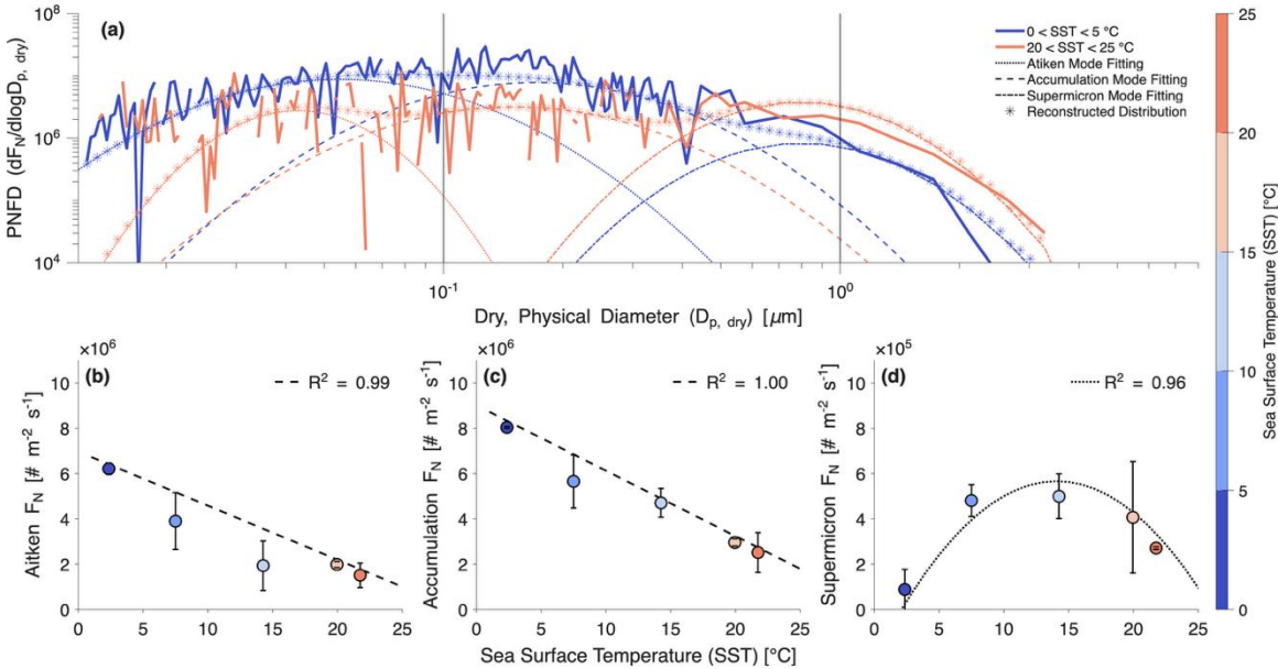
Figure 77: Extreme SST-binned mean PNFD modal decomposition and SST-binned, uncertainty-weighted F_N trends. (a) Average PNFD for 2 °C and 23 °C. Each PNFD is decomposed into three log-normal modes and reconstructed. Weighted least squares linear (dashed lines) and quadratic (dotted lines) regressions of total number flux for the (b) Aitken, (c) accumulation, and (d) supermicron modes.
