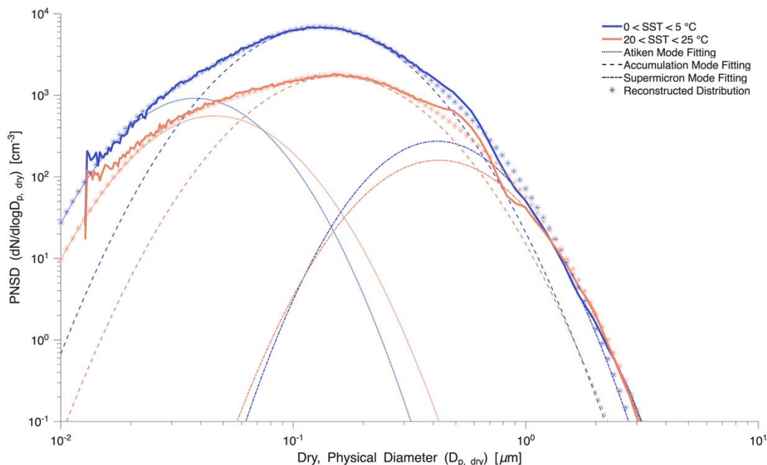
Figure 44: Extreme SST-binned mean PNSD modal decomposition. Average PNSD for the coldest and warmest binned SSTs. Each is decomposed into three log-normal modes and reconstructed.
