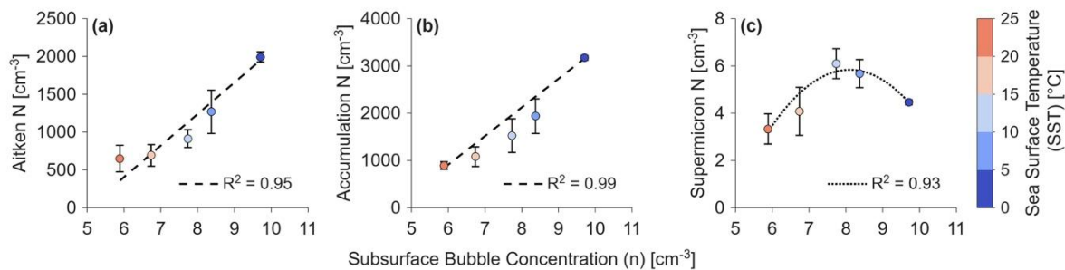
Figure 66: Evaluation of the bubble-SSA correlation using SST-binned, uncertainty-weighted SSA concentrations. Comparison of SSA total number (N) to subsurface bubble concentrations (n), separated by SSA mode: (a) Aitken, (b) accumulation, and (c) supermicron. Weighted least squares regression and resulting best fit lines are shown for linear (dashed) and quadratic (dotted) fits.
