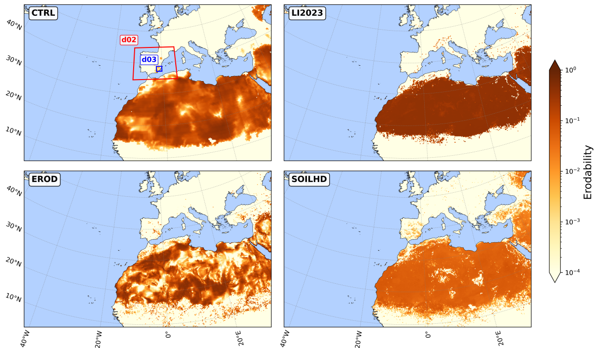
Figure 5. Soil-erodibility fields (sand-layer) Spatial distribution of the 4-sand-fraction soil erodibility for the four experiments (CTRL, LI2023, EROD-HR, and SOILHD) for over domain d01. Unlike Fig. 3, only the sand erodibility layer is shown using a monochromatic color scale. Domains d02 and d03 are represented indicated in the CTRL panel with a by red and a blue rectangle rectangles, respectively.
