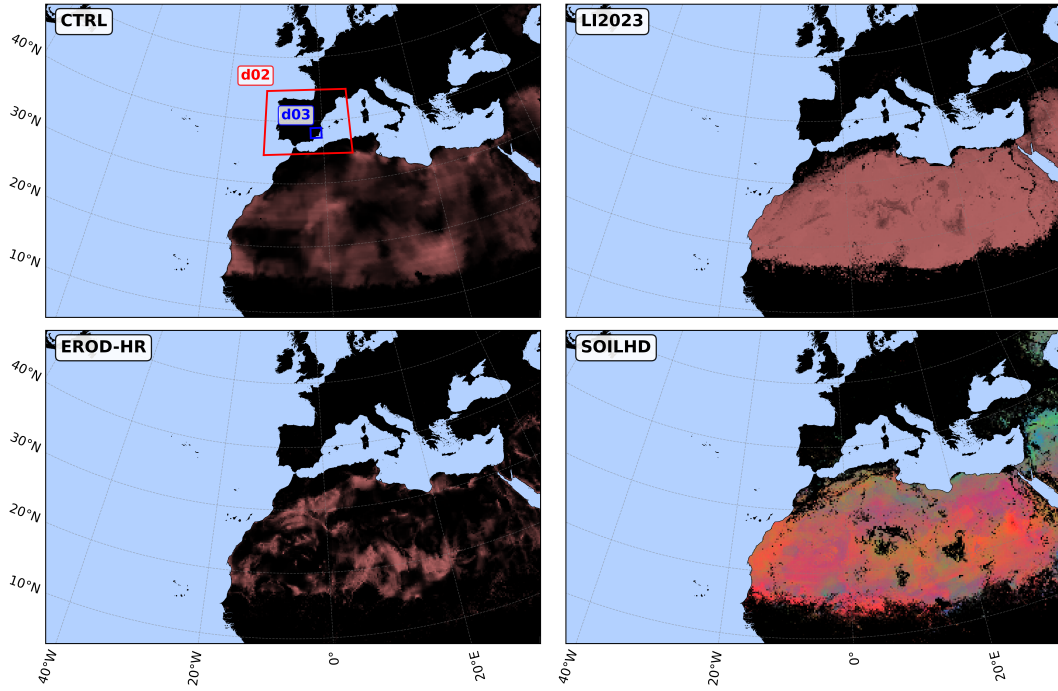
Figure 3. Soil erodibility fields Three-band (sand-layerRGB) composite representation of soil erodibility for the 4 four experiments (CTRL, LI2023, EROD-HR, and SOILHD) for over domain d01. The red, green, and blue channels represent the erodibility of the sand, silt, and clay fractions, respectively. The SOILHD experiment shows a distinct color distribution resulting from its different soil-fraction erodibility dataset. Domains d02 and d03 are indicated in the CTRL panel by red and blue rectangles, respectively.
