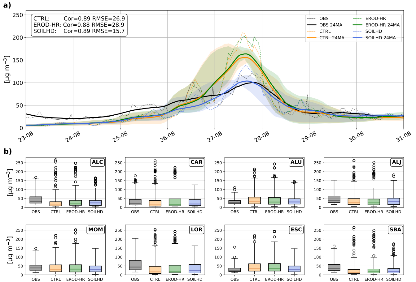
Figure 11. Boxplots for Correlation a) Site-averaged PM_{10} time series (left dashed lines) and relative RMSE-24-hour moving average series (right solid lines) distributions for every simulation period by experiment observations (black) and CTRL (orange), EROD-HR (green), and SOILHD (blue) experiments obtained by bilinearly interpolating the model experiments to each SINCLAIR station location. For a given dataset series, the PM_{10} span across all stations is also represented (light colors). The metrics of every dataset are displayed in the top-left corner of the plot. b) Boxplots with the interpolated PM_{10} values for every station and dataset. Outlier values are represented with circles.
