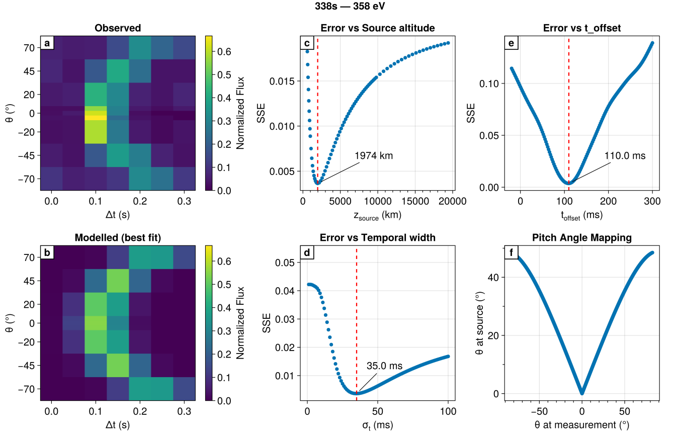
Figure 3. (a) Observed pitch-angle–time dispersion in the 358 eV slice of the event seen at 338 s in Figure 1. The total flux in each pitch-angle channel has been normalized to 1. (b) Best-fitting simulated dispersion by the forward model, as found by the minimization of the SSE. (c) Variation of the SSE over the parameter z_{source} , for the best values of \sigma_t and t_{offset} . (d) Variation of the SSE over the parameter \sigma_t for the best values of z_{source} and t_{offset} . (e) Variation of the SSE over the parameter t_{offset} for the best values of z_{source} and \sigma_t . (f) Relation between the pitch-angle of electrons at the source altitude and measurement altitude.
