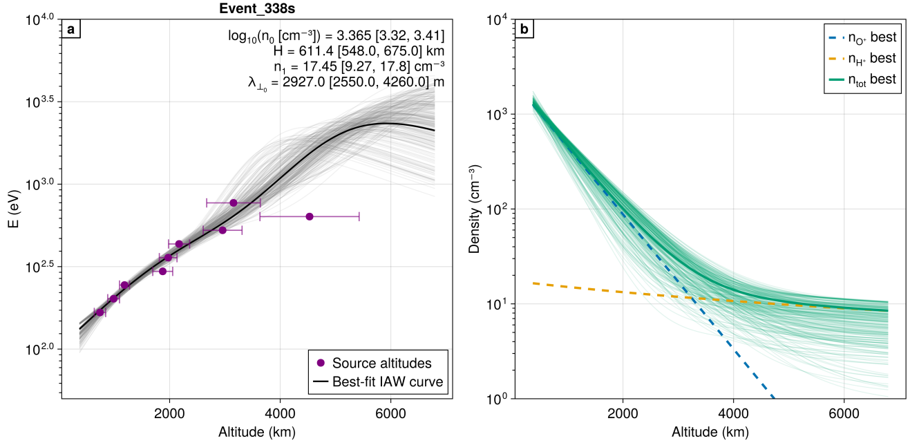
Figure 7. (a) Best-fit IAW speed profile (black curve) to the source altitudes estimated with the pitch-angle method applied to the event at 338 s. The best-fit values of the plasma and wave parameters and the associated uncertainties are indicated in the top-right corner, with the [25th, 75th] percentile interval given in brackets of 250 parameter sets sampled from the fit-error landscape . The faint grey curves correspond to IAW speed profiles computed by varying the parameters around their best value following the linearized error covariance matrix of the estimationsampled parameter sets . (b) Reconstructed density profiles corresponding to the IAW-speed-profiles best-fit parameters of panel a, with faint curves showing the total density of the sampled parameter sets .
