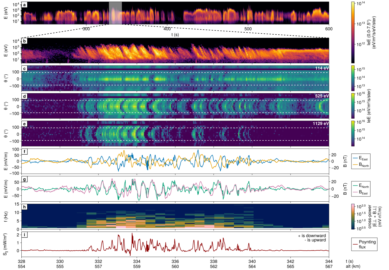
Figure 1. Data from the low-flyer (aNASA 35.040) Electron-EESA and field instruments. (a–b) Differential electron energy flux over time and energy, for 0–7.5° pitch-angle. (b–d–e) Electron-Differential electron energy flux over time and pitch-angle, different panels correspond to different energies (114, 525 and 1129 eV) as indicated in the top right corner of each panel. (ef–g) Perpendicular components of the electric and magnetic fields. DC components have been filtered-out removed using a 6th-order high-pass Butterworth filter with a cut-off frequency of 0.2 Hz. (fh) Cross-power spectrogram |E_{\perp} \times B_{\perp}| of the perpendicular fields (short-time Fourier transform, 2 s Hann window). (i) Field-aligned Poynting flux. Positive values correspond to a downward flux into the ionosphere. The bottom axis is labelled with both flight time since launch (t) and rocket altitude (alt).
