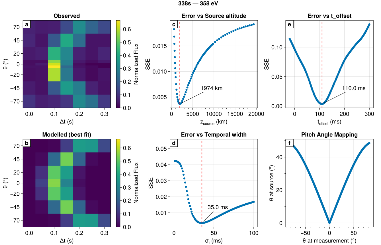
Figure 3. (a) Observed pitch-angle–time dispersion in the 358 eV slice of the event seen at 338 s in Figure 1. The total flux in each pitch-angle channel has been normalized to 1. (b) Best-Best-fitting simulated dispersion by the forward model, as found by the minimization of the SSE. (c) Variation of the SSE over the parameter z_{\text{source}} , for the best values of \sigma_t and t_{\text{offset}} . (d) Variation of the SSE over the parameter \sigma_t for the best values of z_{\text{source}} and t_{\text{offset}} . (e) Variation of the SSE over the parameter t_{\text{offset}} for the best values of z_{\text{source}} and \sigma_t . (f) Relation between the pitch-angle of electrons at the source altitude and measurement altitude.
