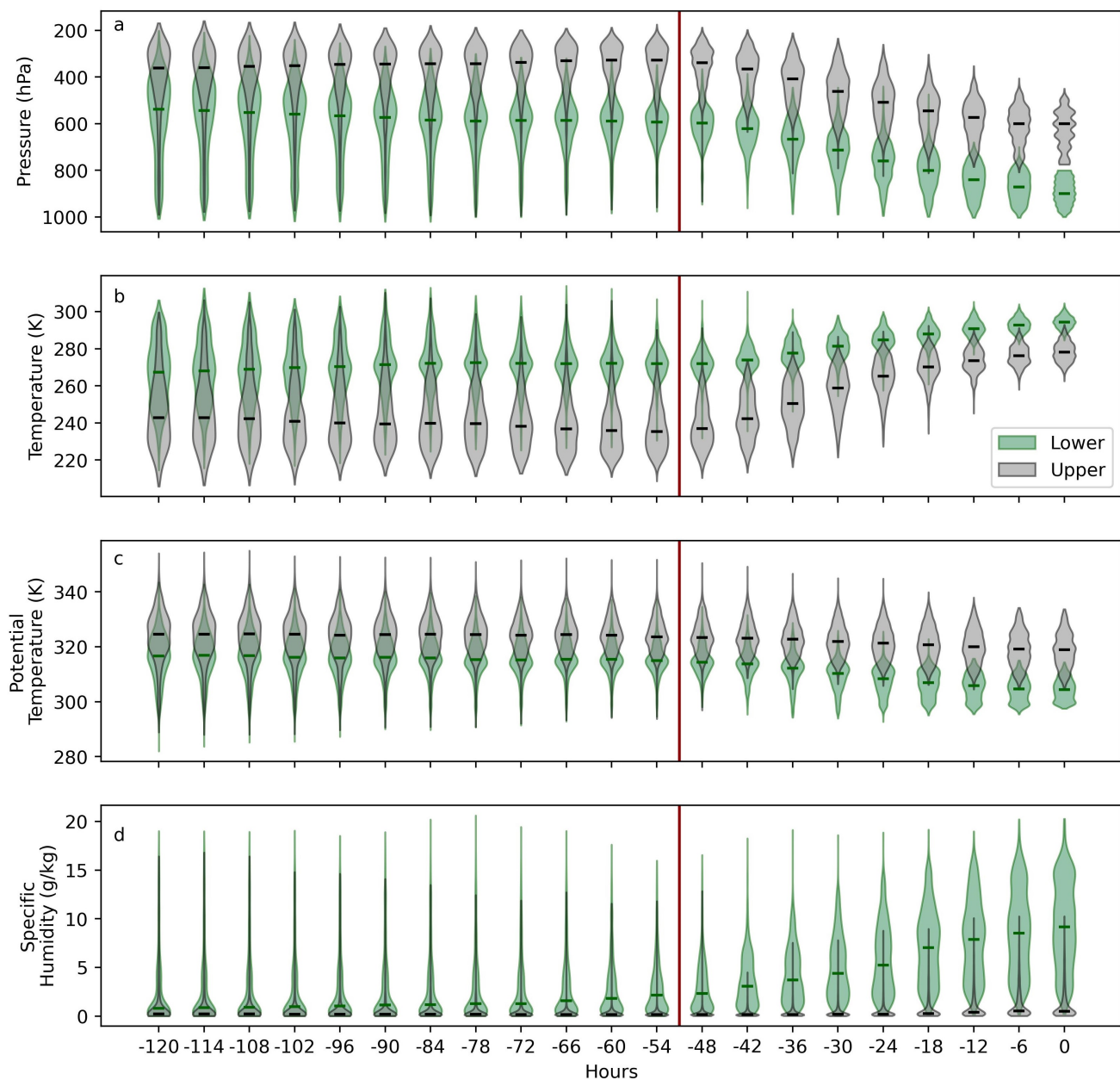
Figure 9. Parcel trajectory properties of the lower ( \geq 800 hPa) and upper ( < 800 hPa) dry intrusions. In each violin plot the median is marked with a horizontal line. The red line marks the separation between the 48 hours after the parcel launch where the descent occurs and the remaining trajectory.
