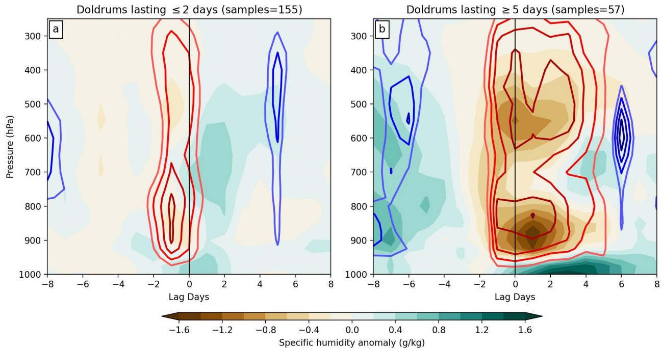
Figure 7. Hovmöller centred on the first day of doldrums formation for Davies Reef (18.75 °S, 147.75 °E) from 1000 hPa to 250 hPa. Specific humidity anomalies (shading) and omega anomalies (contours, every 0.01 Pa s -1 starting from 0.02) for short and long duration doldrums are shown. Red contours denote positive (descending) anomalies while blue denotes negative (ascending) anomalies.
