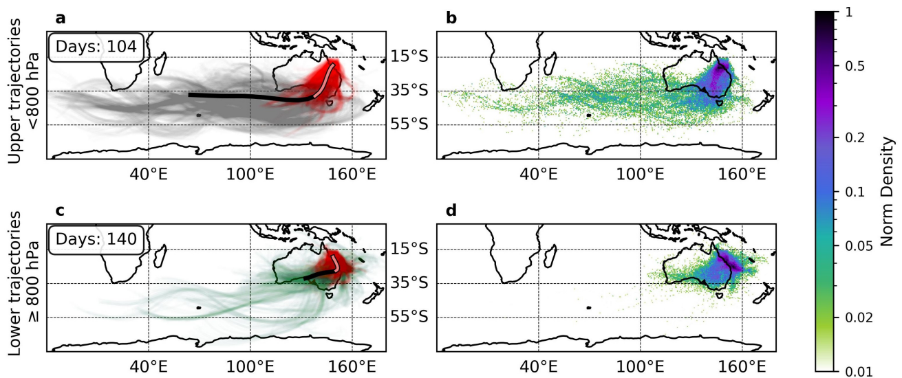
Figure 8. Density plot of the back trajectories launched from Davies Reef that descend >250 hPa in 48 h from their launch time. Trajectories run for 5 days with 6 hourly time steps. The top row shows those that launched from <800 hPa and the bottom row shows trajectories launched from \geq 800 hPa. In panels a and c the red trajectories mark when the parcel is within 48 h of their launch time with the mean trajectory path marked by the solid line (black prior to 48 h, pale red after 48 h). Panels b and d show the normalised density plots of the upper and lower trajectories.
