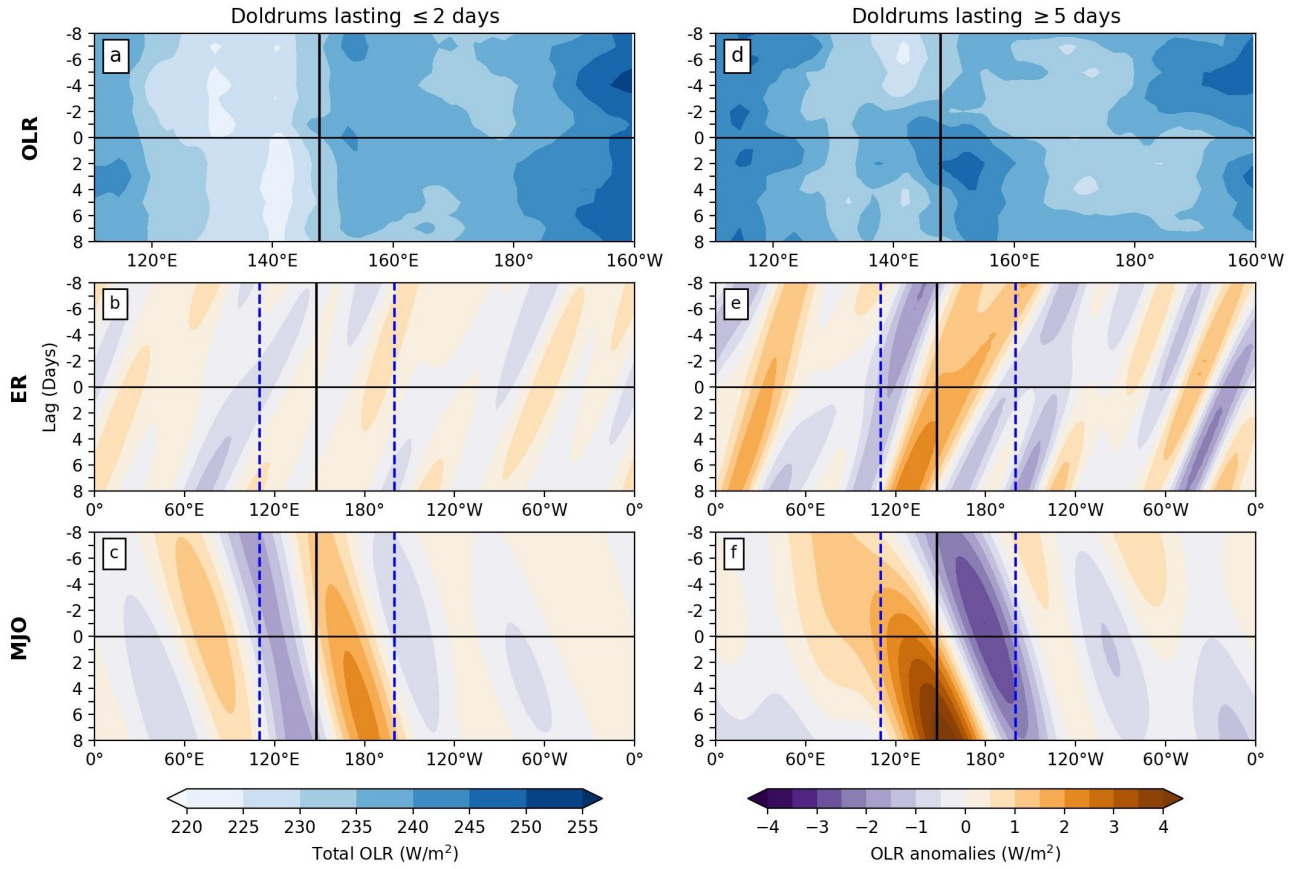
Figure 10. 0-25°S averaged Hovmöller diagrams centred on the first day of the doldrums formation. Top row shows the total OLR between 110°E and 160°W (region marked with blue lines in middle and bottom rows), middle row the ER wave filtered OLR anomalies and bottom row the MJO OLR anomalies. Here positive (negative) anomalies represent suppressed (enhanced) convection. On each panel the vertical line marks the longitude of Davies Reef within the GBR (148°E).
