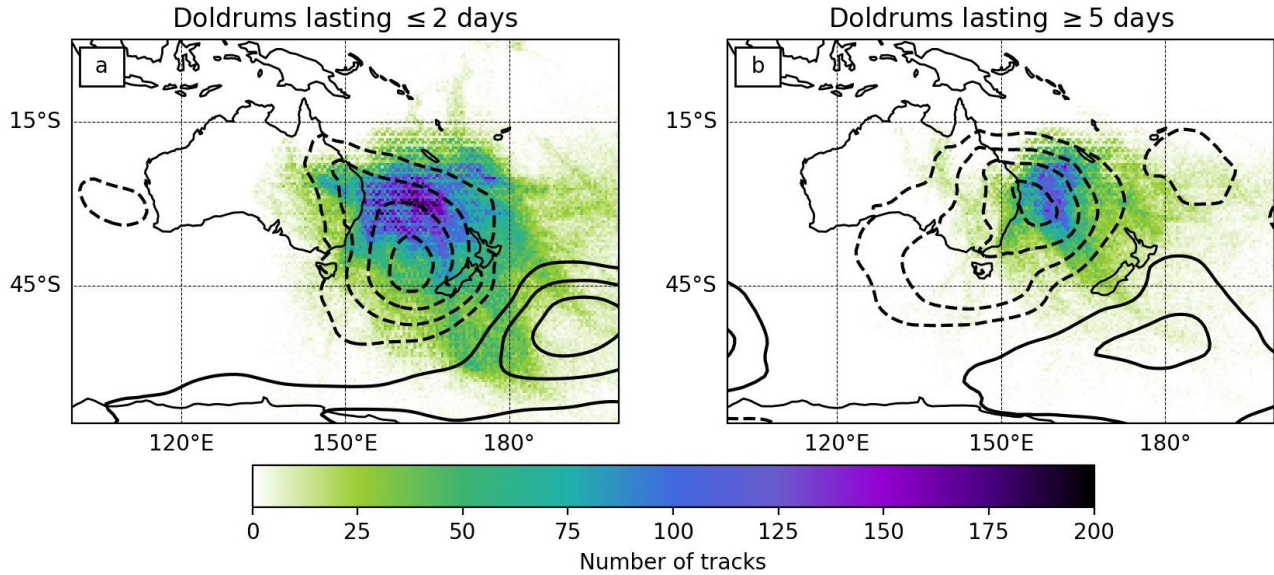
Figure 6. Warm conveyor belt track density (shaded) for short (155 samples) and long (57 samples) doldrums cases showing only the first day of each event. The contours represent the MSLP anomalies (1 hPa intervals, 0 contour removed, dashed is negative, solid is positive)
