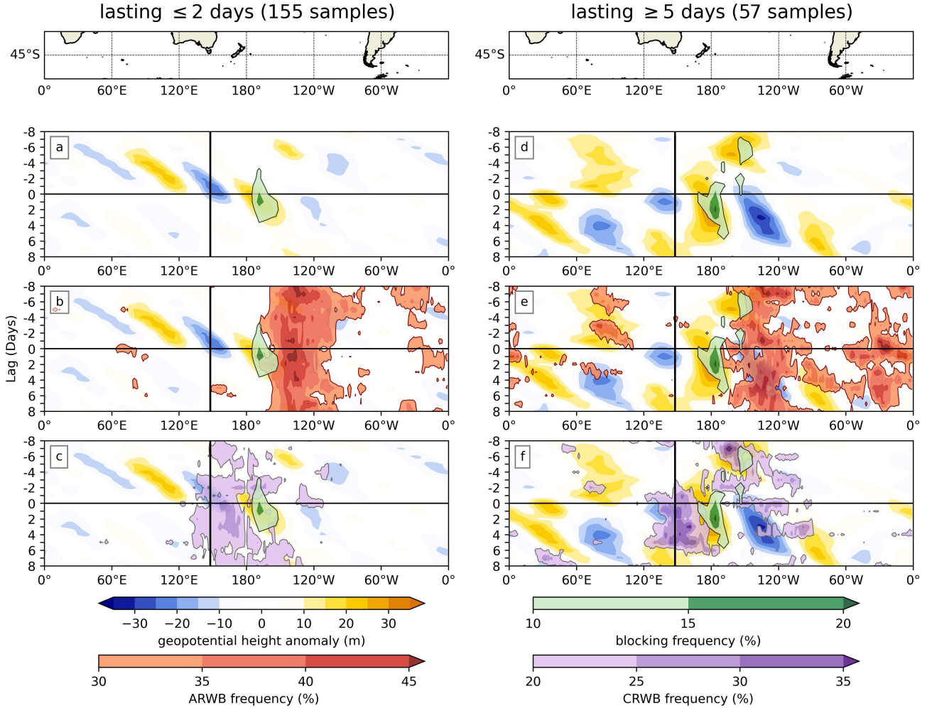
Figure 2. Hovmöller diagrams averaged over 24°S–66°S for lead-lag composites of 500 hPa geopotential height anomalies (blue/yellow), blocking frequency (green, a , d ), anticyclonic Rossby wave breaking (ARWB) frequency (red, b , e ) and cyclonic Rossby wave breaking (CRWB) frequency (purple, c , f ). All lead-lag composites are centred on the first day of the doldrums formation (day 0, horizontal line). The vertical line marks the longitude of Davies Reef and the GBR (148°E).
