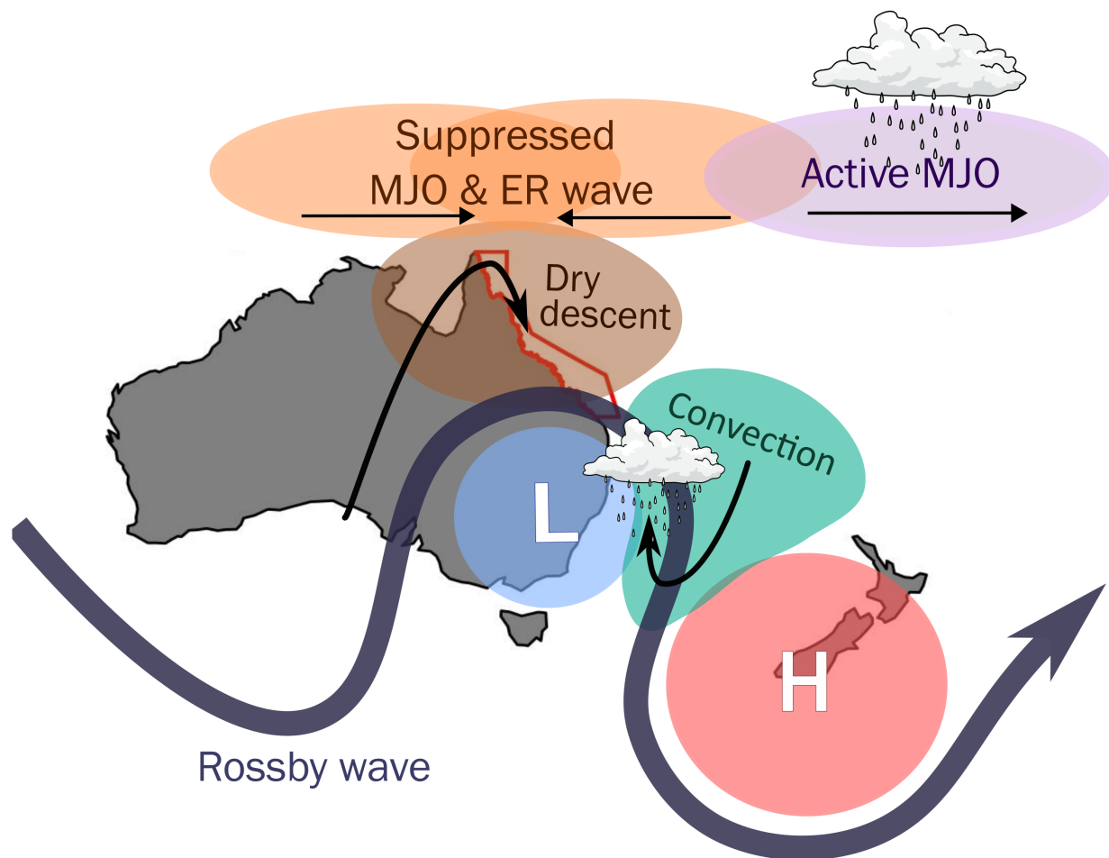
Figure 12. Schematic of persistent doldrums processes over the Australian region
