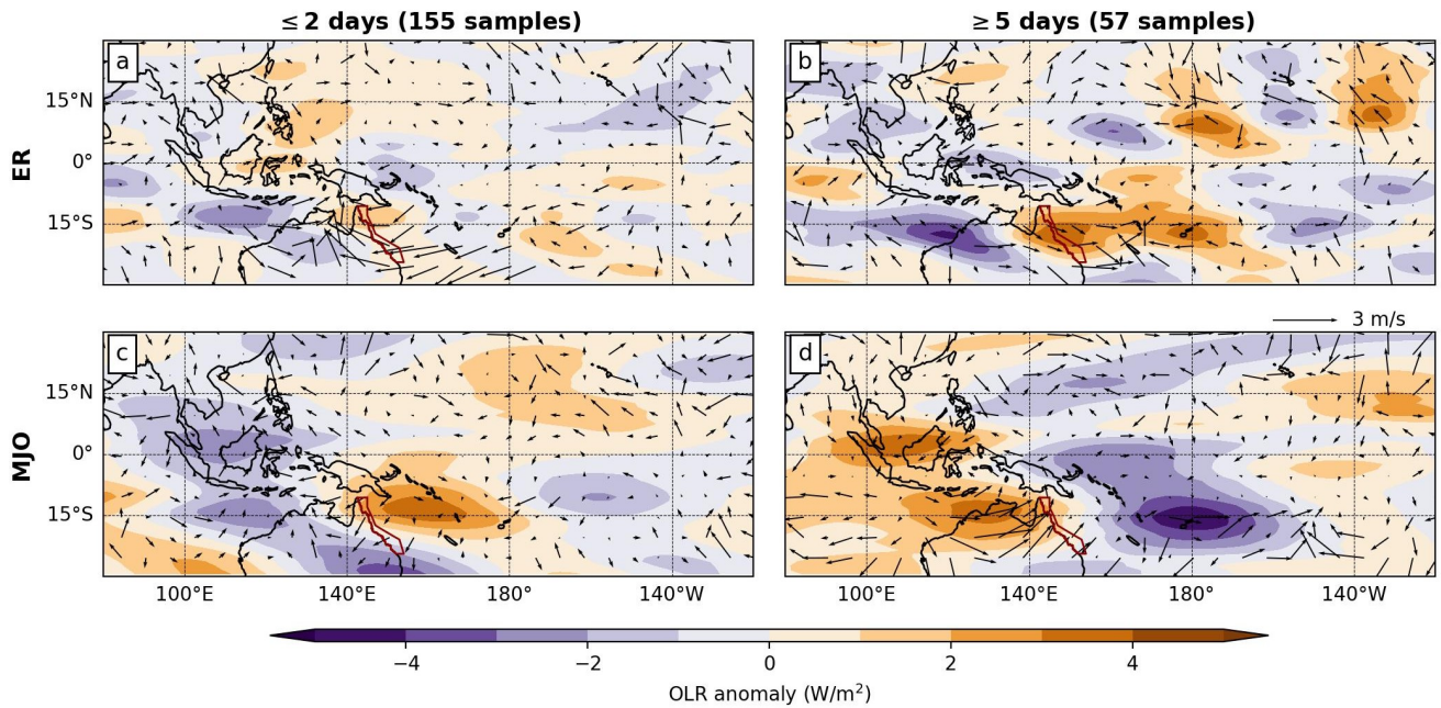
Figure 11. OLR anomalies for the Equatorial Rossby wave (top row) and MJO (bottom row) for short and long duration doldrums. The GBR outline is marked in red. ERA5 850 hPa wind anomalies are composited using only the days where there was a suppressed wave over the GBR giving 43 samples (a), 26 samples (b), 46 samples (c) and 26 samples (d). A quiver key is found above (d).
