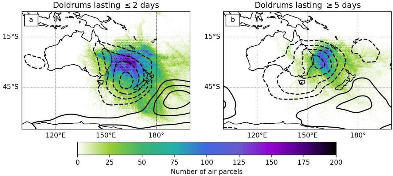
Figure 6. Warm conveyor belt track-air parcel density (shaded) for short (155 samples) and long (57 samples) doldrums cases showing only the first day of each event. The contours represent the MSLP anomalies (1 hPa intervals, 0 contour removed, dashed is negative, solid is positive).
