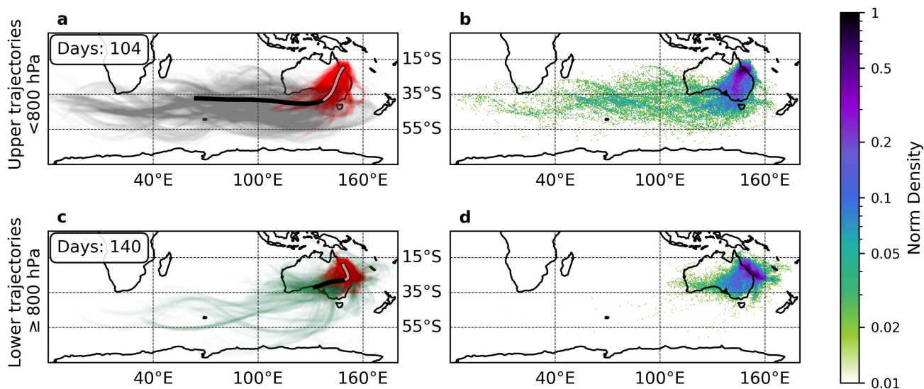
Figure 8. Density plot of the back trajectories launched from Davies Reef that descend >250 \text{ hPa} in 48 h from their launch time. Trajectories run for 5 days with 6 hourly time steps . The top row shows those that launched from <800 \text{ hPa} and the bottom row shows trajectories launched from \geq 800 \text{ hPa} . In panels a and c the red trajectories mark when the parcel is within 48 h of their launch time with the mean trajectory path marked by the solid line ( black prior to 48 h, pale red after 48 h ). Panels b and d show the normalised density plots of the upper and lower trajectories.
