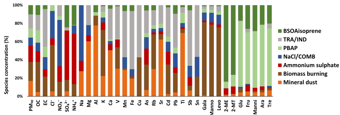
Figure S2. Fingerprints of identified factors in Belgrade; Biomass burning (BB); Long range transport and local combustion (NaCl/COMB); Mineral dust (MD); Primary biological aerosol (PBAP); Biogenic secondary organic (BSOA Isoprene ); ammonium sulfate; Traffic/ Industry (TRA/IND); Gala –galactosan, Manno – mannosan, levo – levoglucosan, 2-ME – 2-methylerythritol, 2-methylthreitol, Glu – glucose, Fru – fructose, Manni – mannitol, Ara – arabitol, Tre – trehalose.
