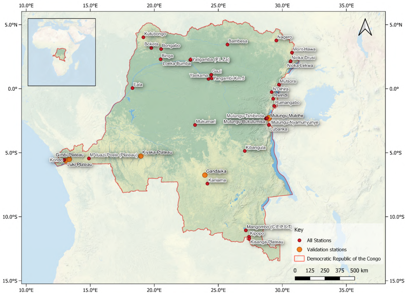
Figure A3. Locations of weather stations in the DRC whose records are archived at the INERA-Section de Climatologie in Yangambi. Red circles show the full station network, while orange circles highlight the subset of stations for which manually transcribed reference data were available and used for validation in Sect. 2.4.1 (Background map courtesy of ESRI National Geographic | Powered by Esri).
