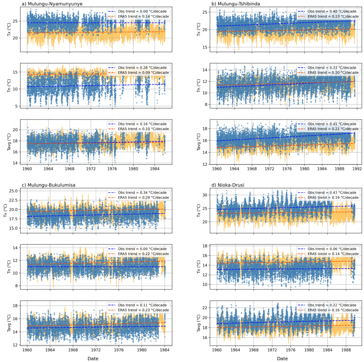
Figure G4. Comparison of trends in daily maximum, minimum and average temperatures at stations: a) Mulungu-Nyamunyunye (S 2°18' E 28°48'), b) Mulungu-Tshibinda (S 2°19' E 28°45'), c) Mulungu-Bukulumisa (S 2°20' E 28°43'), and d) Nioka-Drusi (N 2°09' E 30°39') in the DRC. Blue dots represent daily values of observed maximum, minimum and average temperatures, while solid yellow lines show the ERA5-Land timeseries. The dotted dark blue and orange lines indicate Theil–Sen trend estimates for each variable for observations (Obs) and ERA5-Land, respectively, with the corresponding slope (°C/decade) shown in the top left legend. The observations include both automatically transcribed records using MeteoSaver and manually transcribed records previously available at INERA. The trends are estimated using values where both the ERA5-Land data and transcribed observations are available. Note that these stations have different start and end years.
