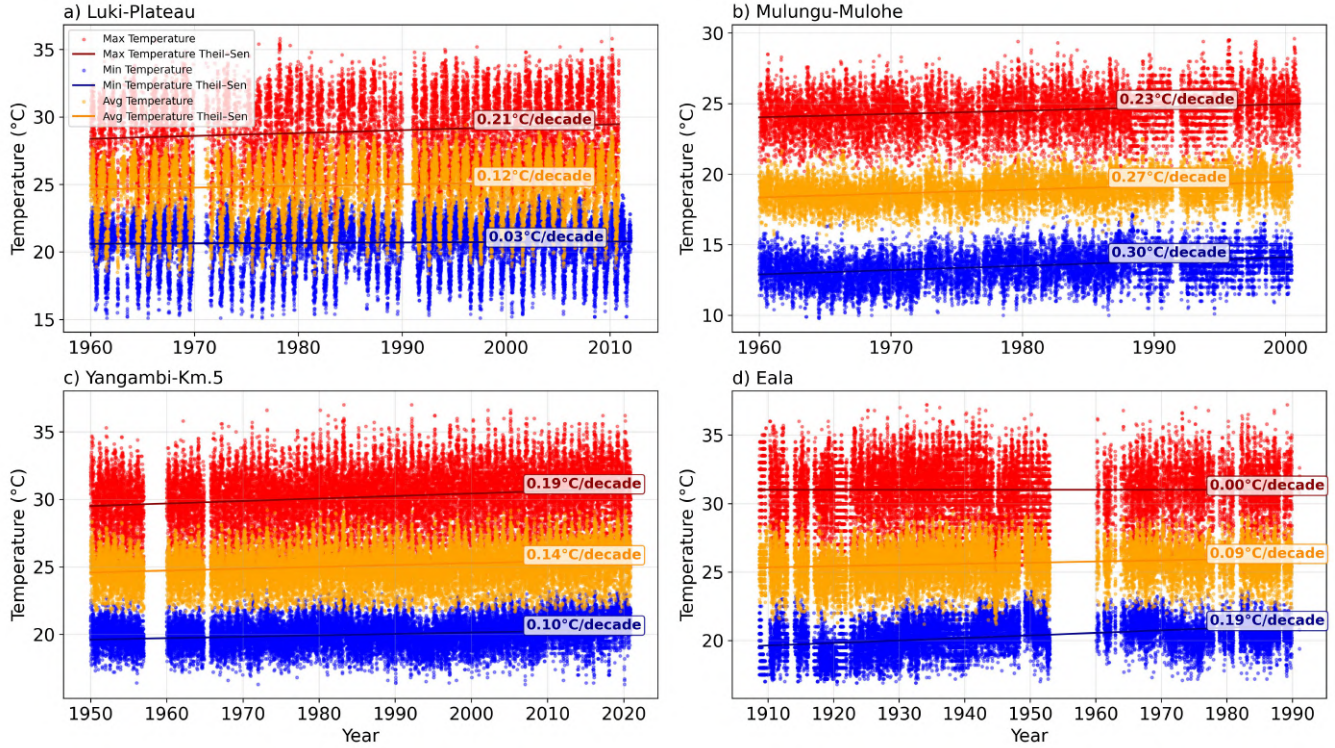
Figure 7. Daily temperature trends at stations: a) Luki-Plateau (S 5°37', E 13°06'), b) Mulungu-Mulohe (S 2°18', E 28°47'), c) Yangambi-Km.5 (N 0°46', E 24°29'), and d) Eala (N 0°03', E 18°18') in the DRC. Colored dots represent daily values of maximum ( T_x , red), average ( T_{avg} , orange), and minimum ( T_n , blue) temperatures. Solid lines indicate Theil–Sen trend estimates for each variable, with the corresponding slope (°C/decade) shown at the end of each line. This data includes both automatically transcribed records using MeteoSaver and manually transcribed records previously available at INERA. Note that these stations have different start and end years.
