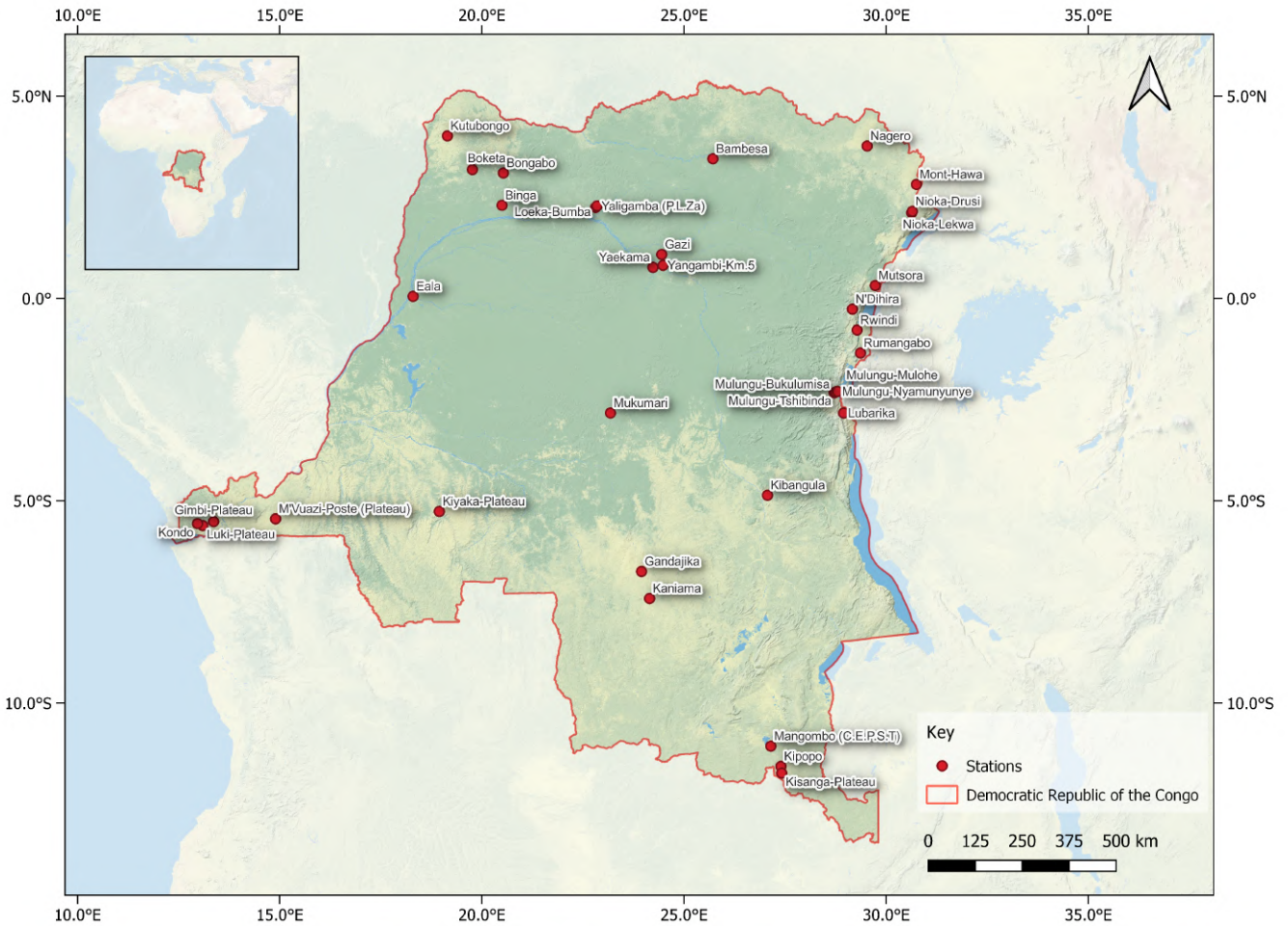
Figure 3. Map showing the location of the 37 weather stations in the DRC whose data is hosted by INERA-Section de Climatologie archives in Yangambi (Background map courtesy of ESRI National Geographic).
