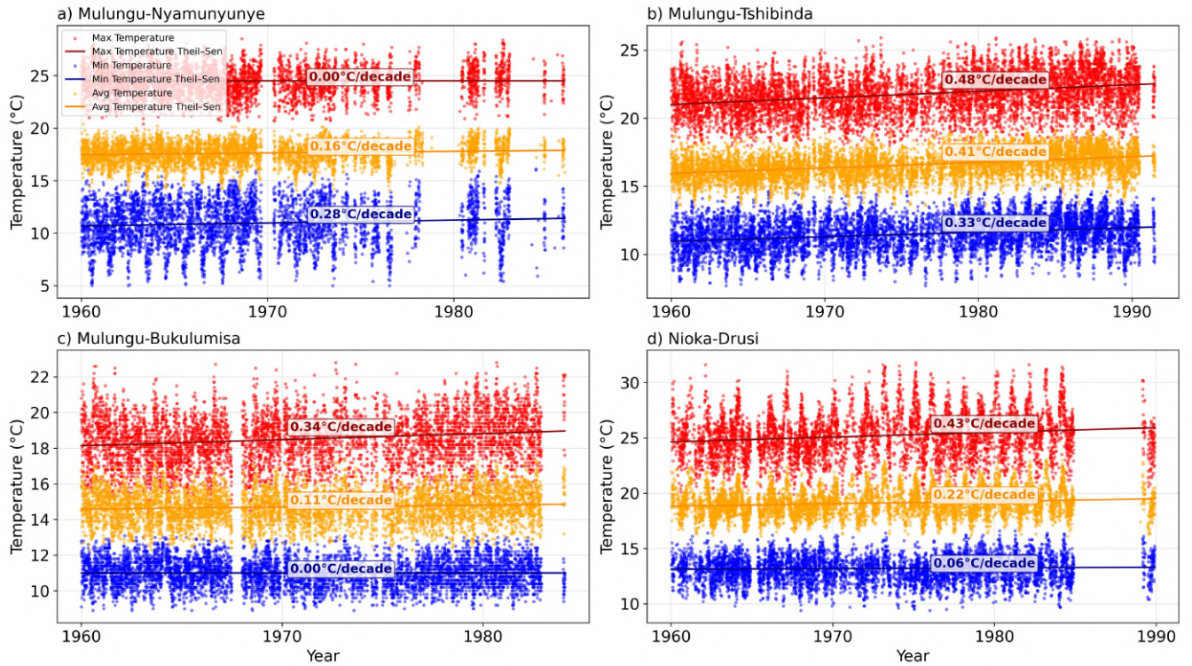
Figure D4. Daily temperature trends at stations: a) Mulungu-Nyamunyunye (S 2°18' E 28°48'), b) Mulungu-Tshibinda (S 2°19' E 28°45'), c) Mulungu-Bukulumisa (S 2°20' E 28°43'), and d) Nioka-Drusi (N 2°09' E 30°39') in the DRC. Colored dots represent daily values of maximum (Tx, red), average (Tavg, orange), and minimum (Tn, blue) temperatures. Solid lines indicate Theil-Sen trend estimates for each variable, with the corresponding slope (°C/decade) shown at the end of each line. This data includes both automatically transcribed records using MeteoSaver and manually transcribed records previously available at INERA. Note that these stations have different start and end years.
