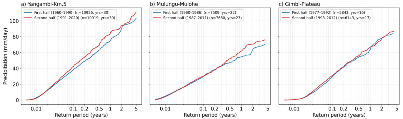
Figure 13. Changes in daily precipitation (P) return periods recorded at three stations: a) Yangambi-Km.5 (N 0°46', E 24°29'), b) Mulungu-Mulohe (S 2°18', E 28°47') and c) Gimbi-Plateau (S 5°31', E 13°22'). The blue lines represent the return periods of daily precipitation (in mm/day) during the first half of the available time series at each station, while the red lines represent those during the second half of the period. Note that while two of the stations have the same starting year (1960), one starts from 1977. All three stations differ in their end years.
