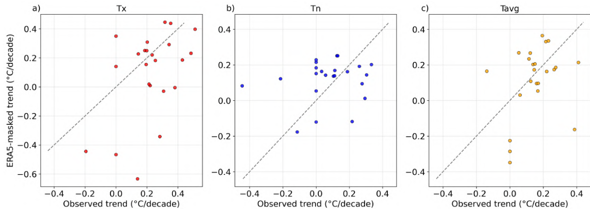
Figure 16. Graphs comparing the observed trends in (a) daily maximum (Tx), (b) daily minimum (Tn), and (c) daily average (Tavg) temperatures from 21 weather stations across the DRC with their corresponding ERA5-Land time series. Note that these stations have different start and end years.
