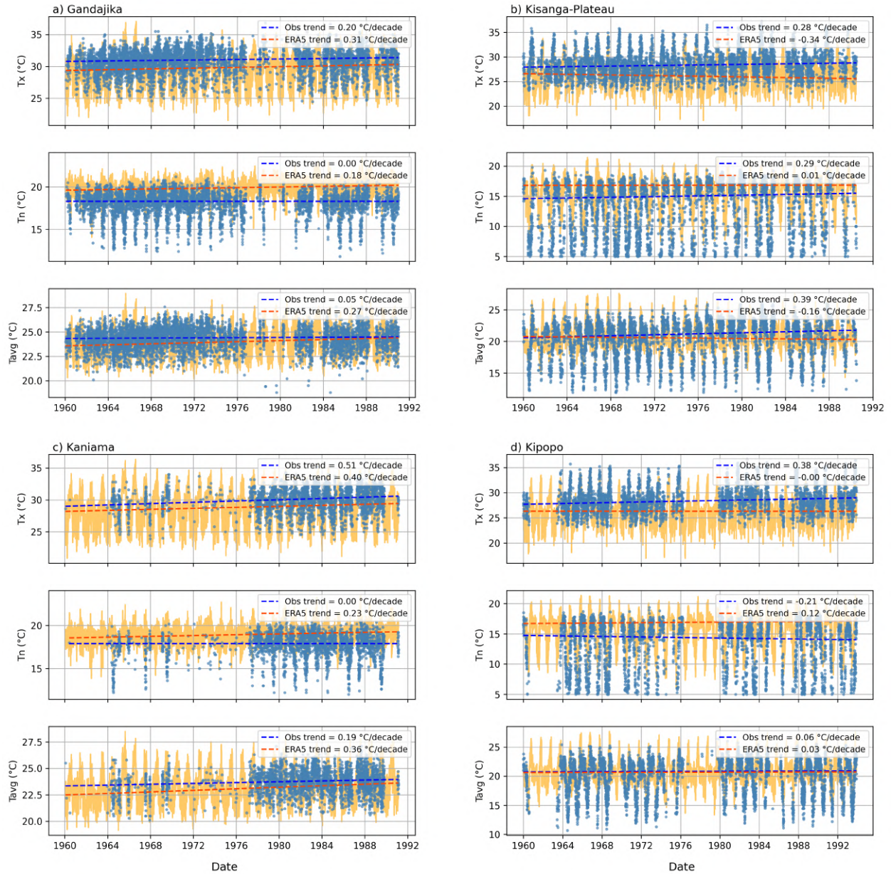
Figure G3. Comparison of trends in daily maximum, minimum and average temperatures at stations: a) Gandajika ( S\ 6^{\circ}45' E\ 23^{\circ}57' ), b) Kisanga-Plateau ( S\ 11^{\circ}44' E\ 27^{\circ}25' ), c) Kaniama ( S\ 7^{\circ}25' E\ 24^{\circ}09' ), and d) Kipopo ( S\ 11^{\circ}34' E\ 27^{\circ}24' ) in the DRC. Blue dots represent daily values of observed maximum, minimum and average temperatures, while solid yellow lines show the ERA5-Land timeseries. The dotted dark blue and orange lines indicate Theil–Sen trend estimates for each variable for observations (Obs) and ERA5-Land, respectively, with the corresponding slope ( ^{\circ}\text{C}/\text{decade} ) shown in the top left legend. The observations include both automatically transcribed records using MeteoSaver and manually transcribed records previously available at INERA. The trends are estimated using values where both the ERA5-Land data and transcribed observations are available. Note that these stations have different start and end years.
