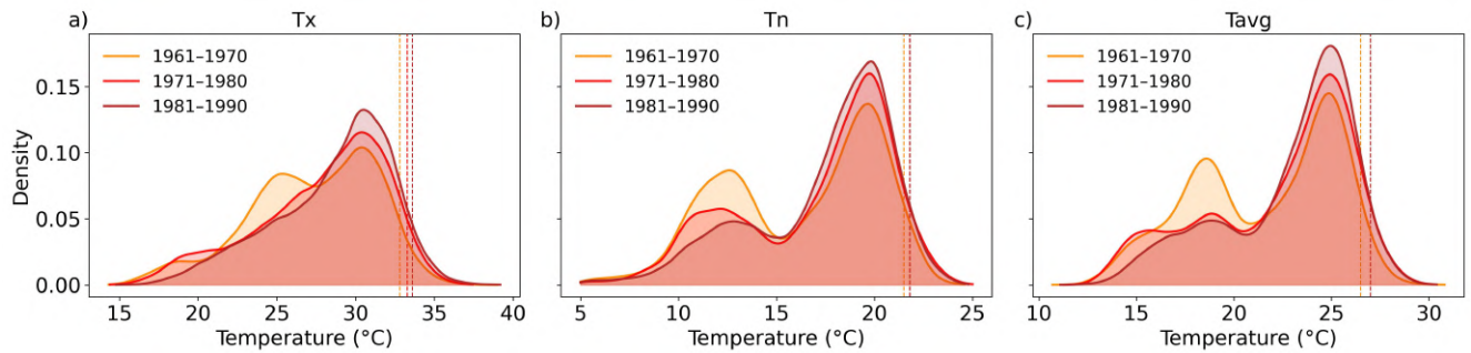
Figure 10. Decadal shifts in temperature distributions based on an aggregated dataset of 37 stations in the DRC for the period 1961 to 1990. The aggregated distributions were obtained by pooling all available QA/QC-confirmed station-day observations across stations during 1961–1990; no additional station-level weighting was applied. Kernel density estimates of daily maximum (Tx), minimum (Tn), and average (Tavg) temperatures are shown for each decade: 1961–1970 (yellow), 1971–1980 (red), and 1981–1990 (maroon). Vertical dashed lines indicate the 95th percentile values for each decade, illustrating the progressive rightward shift in temperature extremes over time.
