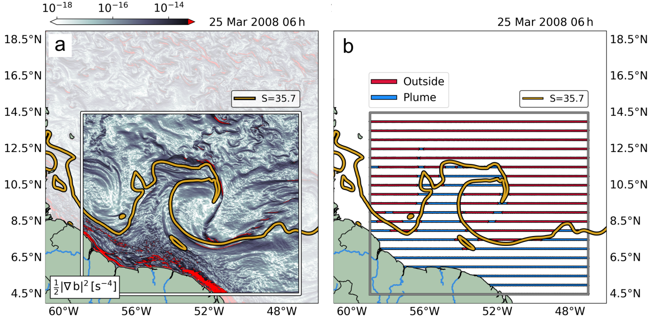
Figure 5. (a) Model spatial distribution of buoyancy sharpness B = \frac{1}{2} |\nabla b|^2 and the separation between PLUME and OUTSIDE regions using the 0.25 quantile of the salinity distribution. (b) Latitudinal transects used to compute the magnitude of surface density gradients within the PLUME and OUTSIDE.
