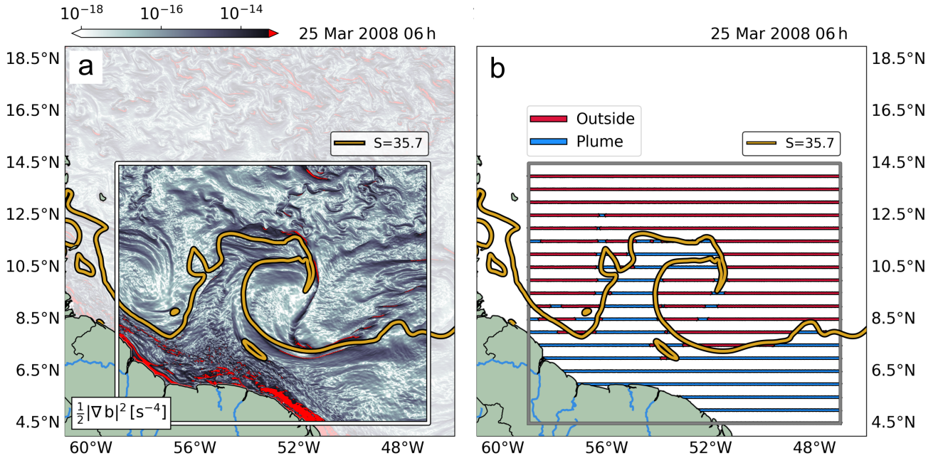
Figure 5. (a) Model spatial distribution of buoyancy sharpness B = \frac{1}{2}|\nabla b|^2 and the separation between PLUME and OUTSIDE regions using the 0.25 quantile of the salinity distribution. (b) Latitudinal transects used to compute the magnitude of surface density gradients within the PLUME and OUTSIDE.
