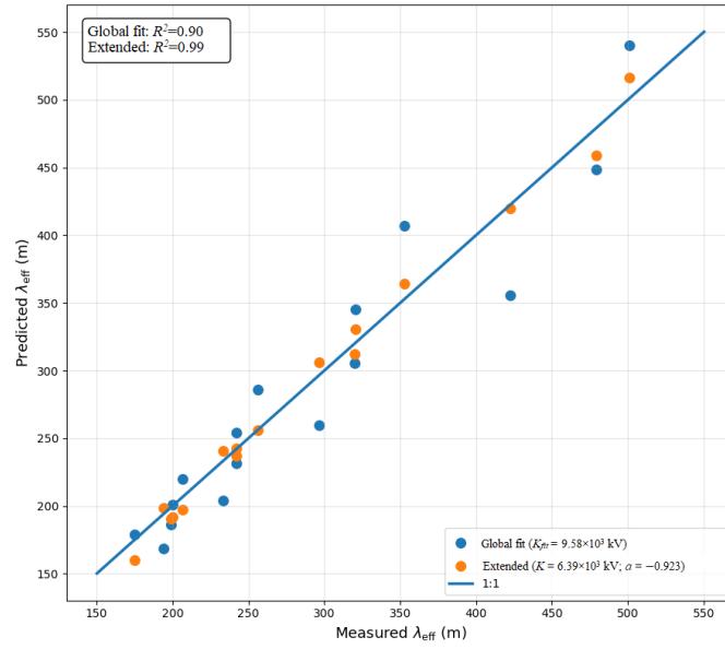
242 Figure 2. Parity comparison between the effective avalanche lengths obtained from the CORSIKA simulations 243 and those predicted by the global and extended fits.
