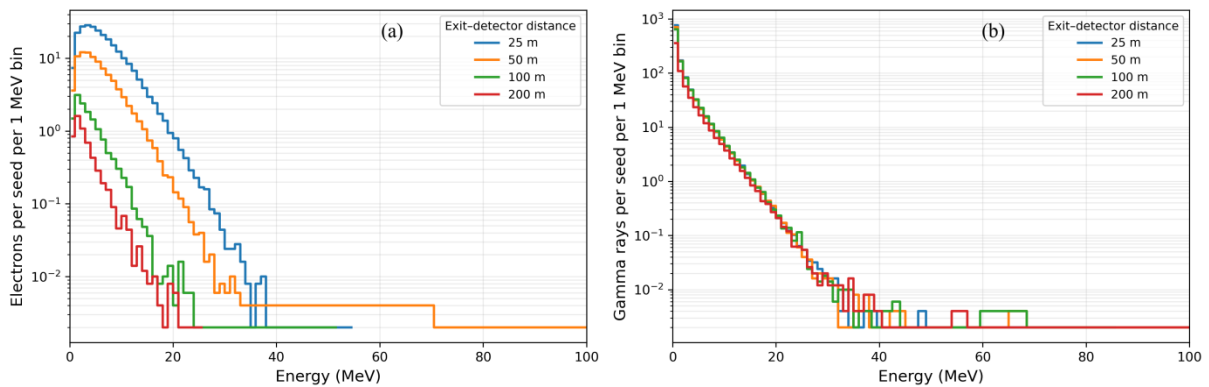
251 Figure 3. Electron (a) and gamma-ray (b) energy spectra for detector levels located 25, 50, 100, and 200 m 252 below the lower boundary of the electric field for the Aragats configuration. The spectra are normalized per 253 injected seed electron.
