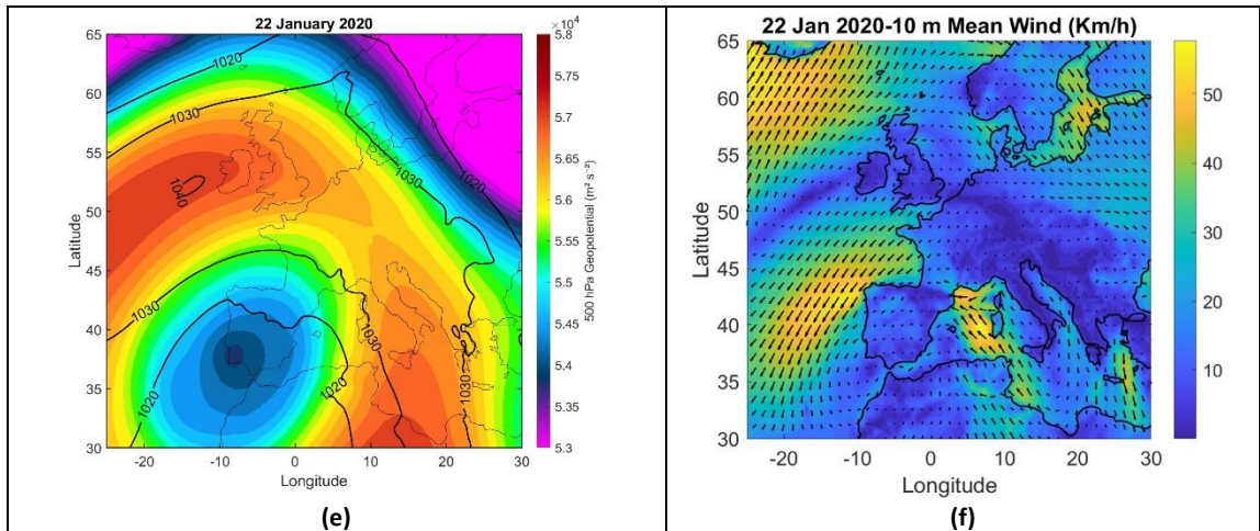
Figure 2: Sea level pressure and 500 hPa geopotential (a, c, e) and mean wind speed (b, d, f) for January 20, 21 and 22, 2020.
