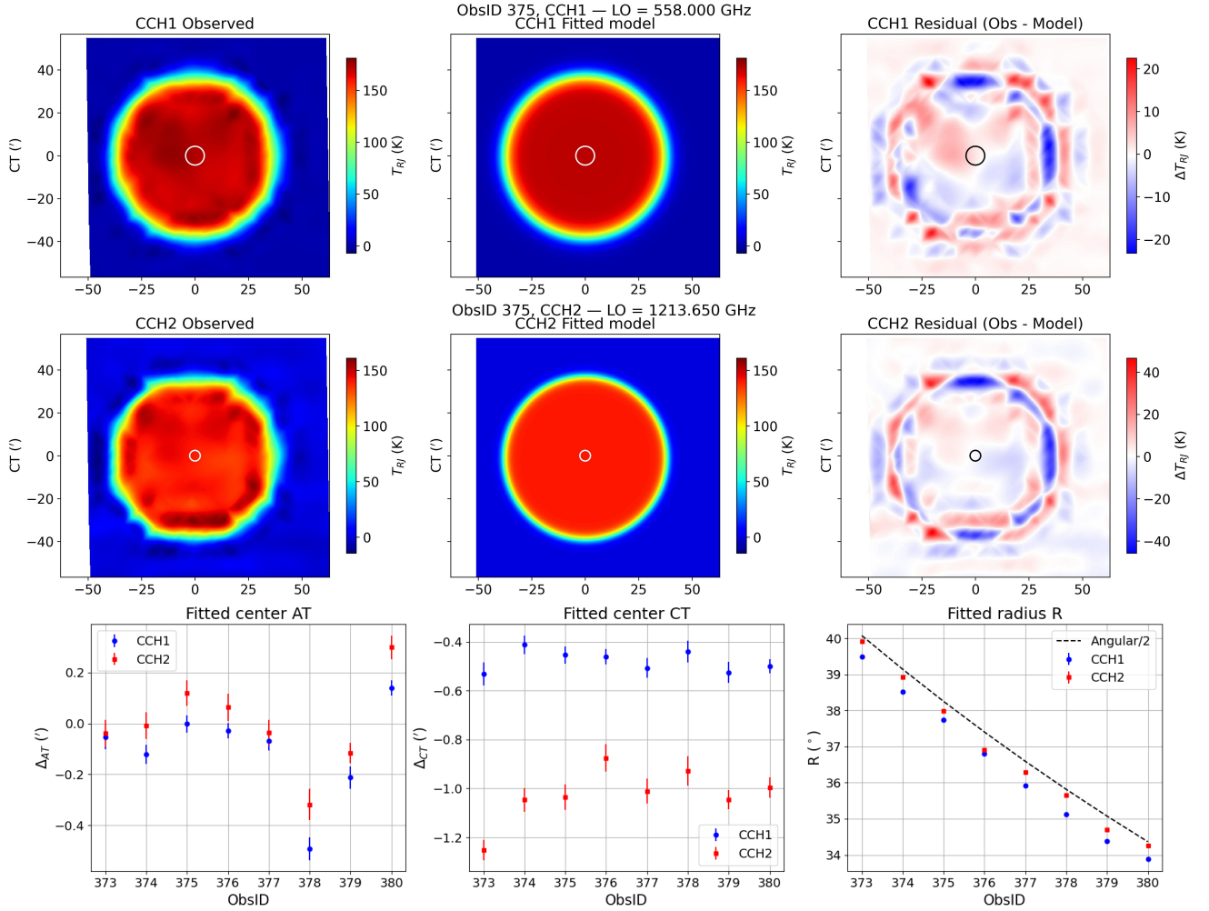
Figure 4. Circular disk fitting for 2D maps of Earth. The first two rows show from left to right the observation, model fit, and the residuals for ObsID 375. The first two rows correspond to the two instrument channels. The last row shows a comparison of selected fit parameters between ObsIDs and in the last panel, the dashed line Angular/2 represents the Earth angular radius at the beginning of the observations. The white circles at the centers represent the beam sizes.
