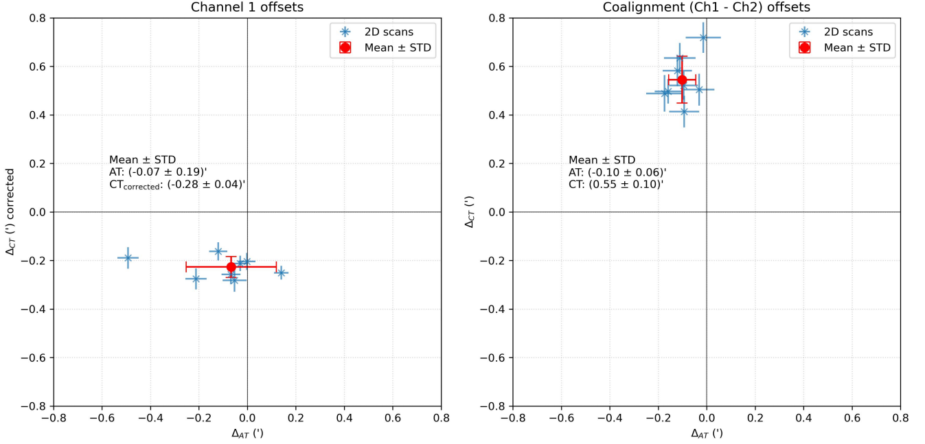
Figure 5. A 2D visualisation of the fitted pointing offsets determined from 2D map data observed during LEGA. The fitted parameters are corrected for the change in target angular size during the \sim 1 hour observation time. Detailed values can be found in Table B1.
