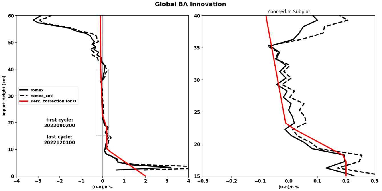
Fig. 1: Global bending angle normalized innovation for the ROMEX experiment (“romex”) and the control experiment (“romex_cntl”) as a function of impact height. The empirical bias correction model derived from all ROMEX RO bending angle observations is also shown (red lines). The right panel shows a zoomed-in view of the left panel for impact heights between 15 and 40 km (grey box).
