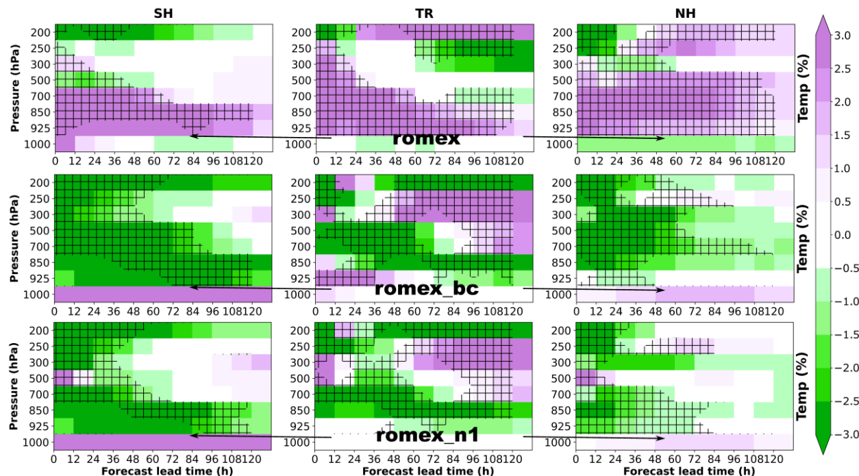
285 Fig. 7: Same as Fig. 5, but for temperature.
