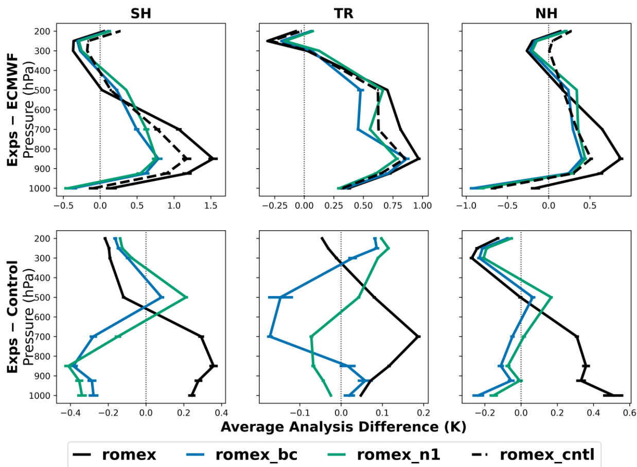
285 Fig. 7: Same as Fig. 5, but for temperature.
