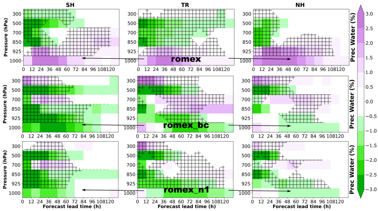
Fig. 9: Same as Fig. 5, but for precipitable water.
