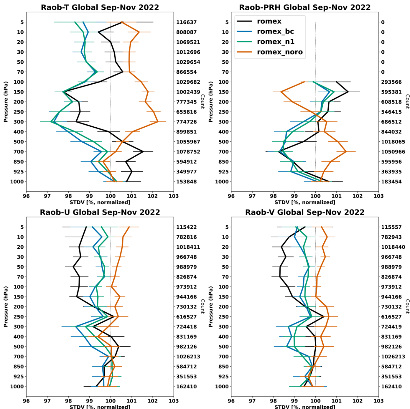
Fig. 3. Change in standard deviation of observed minus background for radiosondes temperature, pseudo relative humidity (PRH), and zonal and meridional wind for ROMEX (“romex”), bias-corrected romex (“romex_bc”), adjusting the first refractivity coefficient ROMEX experiment (“romex_n1”), and the one without RO data (“romex_noro”) experiment relative to the ROMEX control experiment (“romex_cntl”) from September to November 2022. The number of observations is indicated on the vertical axis to the right, and the horizontal bars represent the 95% significance level.
