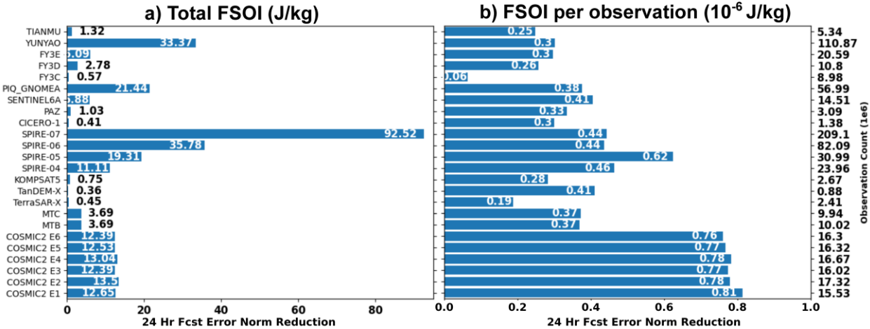
Fig. 4: (a) Total forecast sensitivity to observation impact (FSOI, J/kg) and (b) per observation FSOI for all the ROMEX missions from September to November 2022 from the romex_n1 experiment. Spire instrument receiver IDs are grouped as follows: Spire 04 (99–102), 205 Spire 05 (103–117), Spire 06 (118–125), and Spire 07 (126–169).
