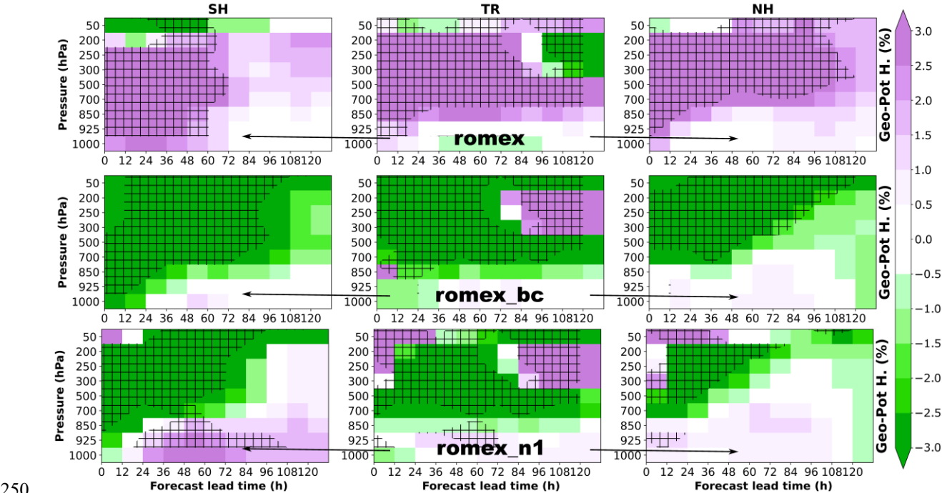
250 Fig. 5: Percentage change in root-mean-square-error (RMSE) reduction for geopotential height forecasts in the “romex”, “romex_bc”, and “romex_n1” experiments relative to the control, verified against ECMWF analyses for September–November 2022. Forecast RMSE is computed every 12 hours for the control and comparison experiment at three distinct regions: Southern Hemisphere (SH, 20°–80°S), tropics (TR, 20°S–20°N), and Northern Hemisphere (NH, 20°–80°N). Green shading indicates improved forecast skill from the assimilation of ROMEX observations, while purple shading signifies degraded skill. Hatched areas denote impacts that are statistically significant at the 95% confidence level. 255
