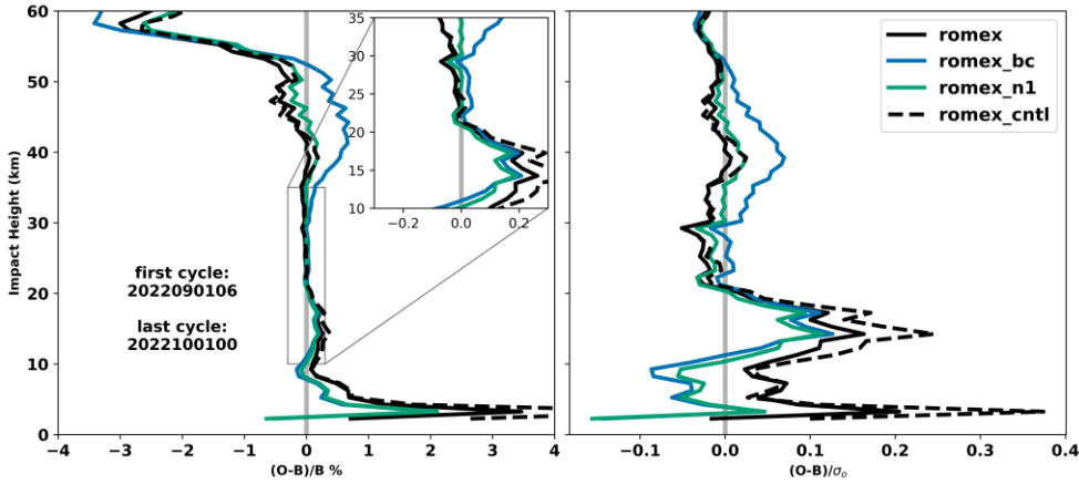
Fig. 2: Global bending angle innovation normalized (a) by the background (B) and (b) by the observation uncertainties error ( \sigma_o ) for the ROMEX experiment (“romex”), bias-corrected ROMEX experiment (“romex_bc”), and adjusting refractivity coefficient ROMEX experiment (“romex_n1”) as a function of impact height.
