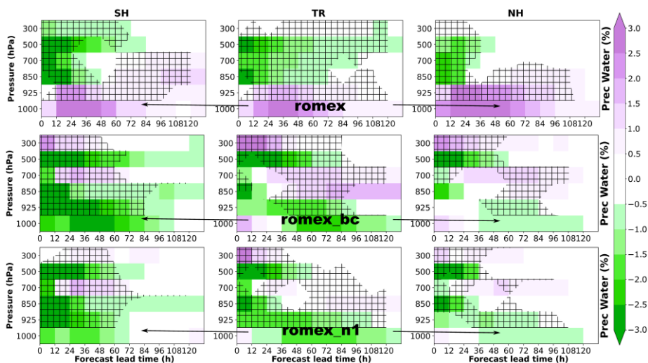
Fig. 9: Same as Fig. 5, but for precipitable water.
