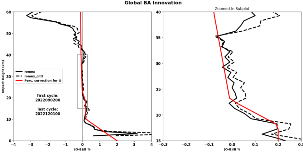
Fig. 1: Global bending angle normalized innovation for the ROMEX experiment (“romex”) and the control experiment (“romex_cntl”) as a function of impact height. The empirical bias correction model derived from all ROMEX RO bending angle observations is also shown (red lines). The right panel shows a zoomed-in view of the left panel for impact heights between 15 and 40 km (grey box).
