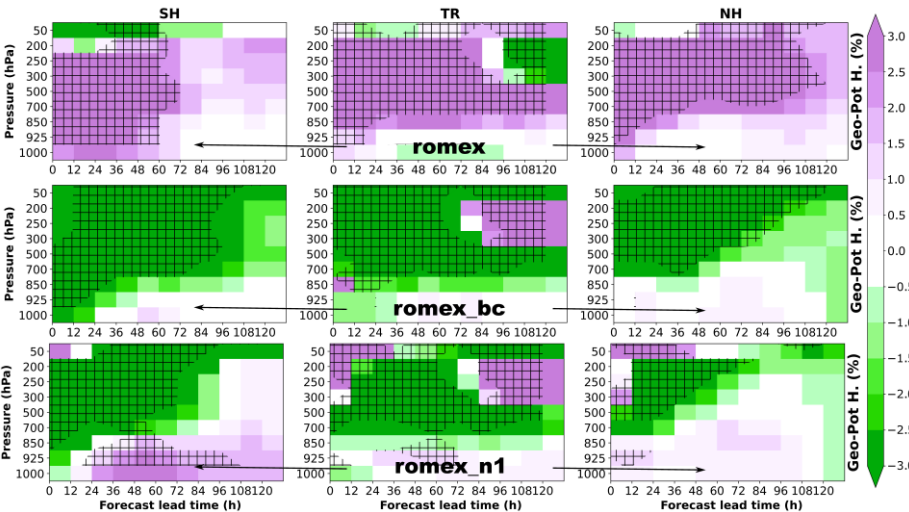
Fig. 5: Percentage change in root-mean-square-error (RMSE) reduction for geopotential height forecasts in the “romex”, “romex_bc”, and “romex_n1” experiments relative to the control, verified against ECMWF analyses for September–November 2022. Forecast RMSE is computed every 12 hours for the control and comparison experiment at three distinct regions: Southern Hemisphere (SH, 20°–80°S), tropics (TR, 20°S–20°N), and Northern Hemisphere (NH, 20°–80°N). Green shading indicates improved forecast skill from the assimilation of ROMEX observations, while purple shading signifies degraded skill. Hatched areas denote impacts that are statistically significant at the 95% confidence level.
