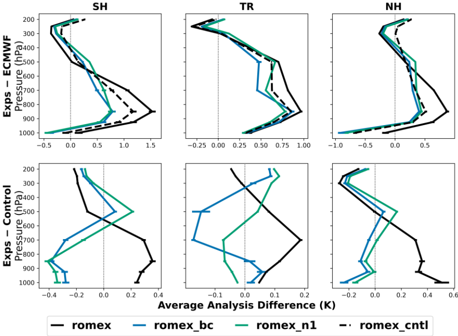
Fig. 7: Same as Fig. 5, but for temperature.
