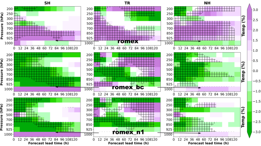
Fig. 7: Same as Fig. 5, but for temperature.
