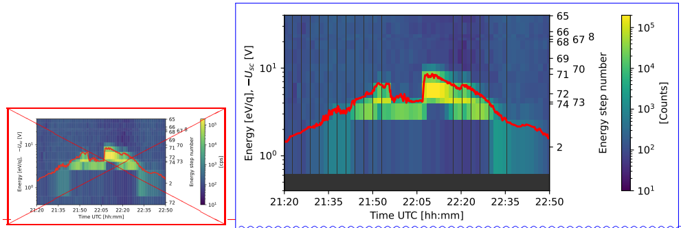
Figure 5. The same energy-time spectrogram as in Fig. 3 after correction of the energy scale. The energy is given in eV/q. The value presented is a sum over all directions of arrival and all masses. The red line is an estimate of the negative of the spacecraft potential (in V) estimated from RPWI observations. The energy step numbers are indicated on the right-side vertical axis.
