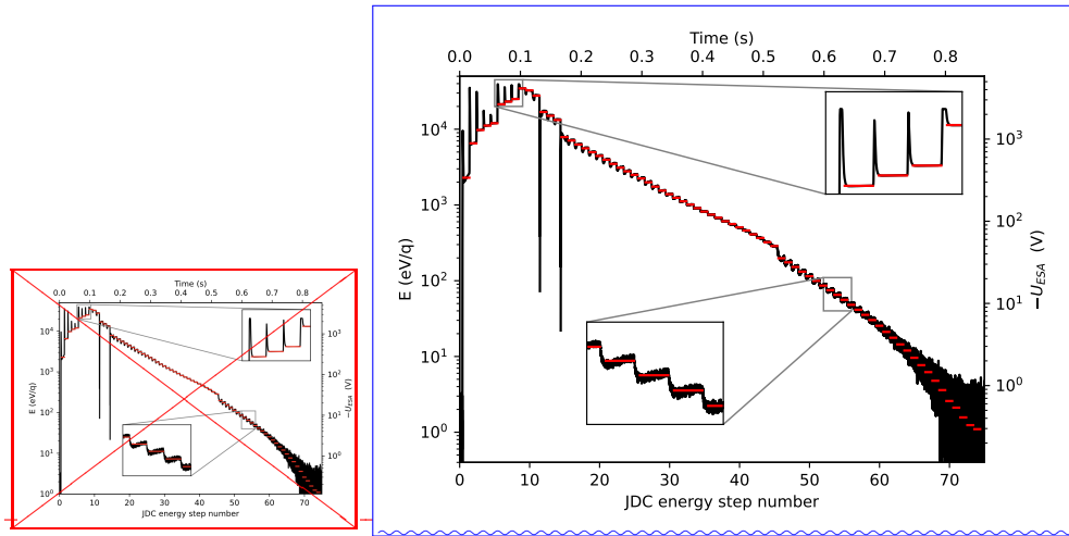
Figure 8. Optimized energy table for the 1 eV-eV to 35 keV-keV range. The other new tables use the same approach with a long and slow downgoing part of the sweep. The step visible at energy bin number 45 is due to a range change in the high voltage power supply.
