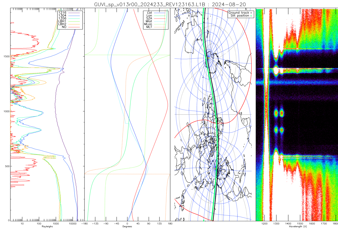
Screenshot from https://guvitimed.jhuapl.edu/index.php/guvi-gallery/lbspec_V013 (year: 2024, day of year: 233, orbit: 123163)
