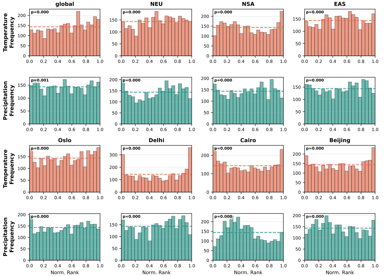
Figure 5. In-sample rank histograms for NorESM2-MM (SSP2-4.5) across multiple regions and variables. A uniform distribution (dashed line) indicates a perfectly representative ensemble. Each panel is annotated with the chi-squared uniformity p-value on the 21-bin count vector ( df = 20 ); values shown in bold indicate p < 0.05 , i.e. formal rejection of the uniformity null.
