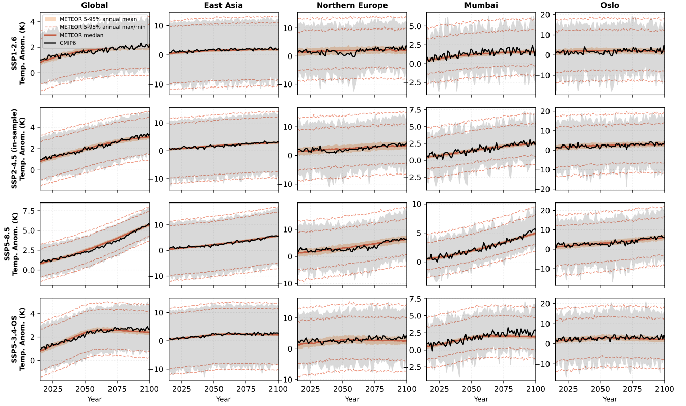
Figure 7. Out-of-sample temperature validation for CNRM-ESM2-1 trained on SSP2-4.5. Each row shows a validation scenario (SSP1-2.6, SSP2-4.5, SSP5-8.5, SSP5-3.4-OS); each column shows a spatial scale (global, East Asia, Northern Europe, Mumbai, Oslo). Orange shading: METEOR 5–95% ensemble range of annual means. Orange dashed lines: 5–95% range of annual maximum and minimum values. Orange solid line: ensemble median of annual means. Black line and grey shading: CMIP6 annual mean and monthly min/max envelope. Results for other models are shown in Supplemental Figures 1–4.
