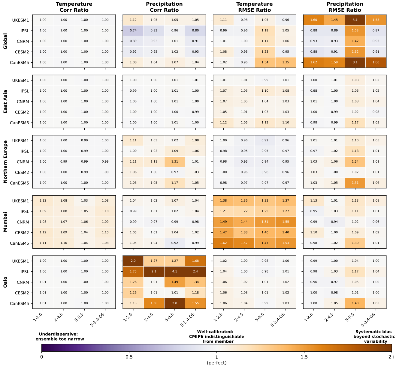
Figure 10. Skill ratio analysis for out-of-sample validation across all spatial scales (rows), models, and scenarios. Each panel shows a grid of model-scenario combinations. Skill ratios are defined such that values >1 (orange) indicate poorer emulation for both metrics: for correlation, ratio = Member-Member / Member-CMIP6; for RMSE, ratio = Member-CMIP6 / Member-Member. Values near 1 (white) indicate CMIP6 is statistically indistinguishable from a METEOR ensemble member; values <1 (purple) suggest ensemble underdispersion. Temperature ratios are consistently near unity; precipitation shows more variability, particularly at global scales where forced response bias is evident.
