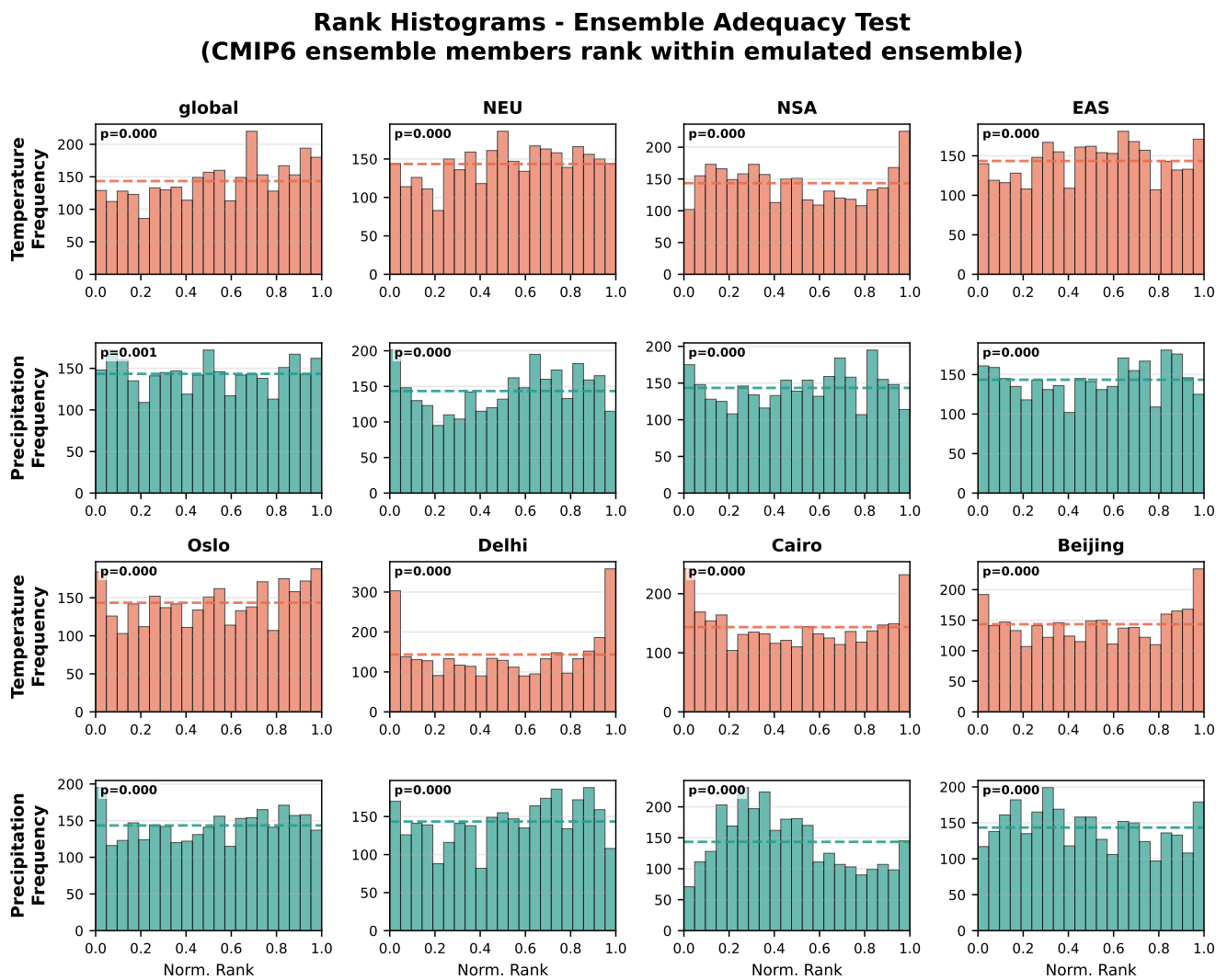
Figure 5. In-sample rank histograms for NorESM2-MM (SSP2-4.5) across multiple regions and variables. A uniform distribution (dashed line) indicates a perfectly representative ensemble. Each panel is annotated with the chi-squared uniformity p-value on the 21-bin count vector (df = 20); values shown in bold indicate p < 0.05 , i.e. formal rejection of the uniformity null.
