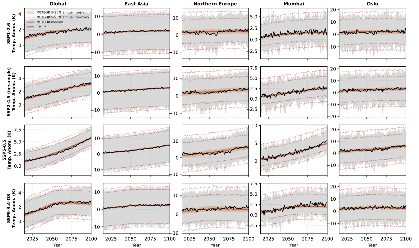
Figure 7. Out-of-sample temperature validation for CNRM-ESM2-1 trained on SSP2-4.5. Each row shows a validation scenario (SSP1-2.6, SSP2-4.5, SSP5-8.5, SSP5-3.4-OS); each column shows a spatial scale (global, East Asia, Northern Europe, Mumbai, Oslo). Orange shading: METEOR 5–95% ensemble range of annual means. Orange dashed lines: 5–95% range of annual maximum and minimum values. Orange solid line: ensemble median of annual means. Black line and grey shading: CMIP6 annual mean and monthly min/max envelope. Results for other models are shown in Supplemental Figures 1–4.
