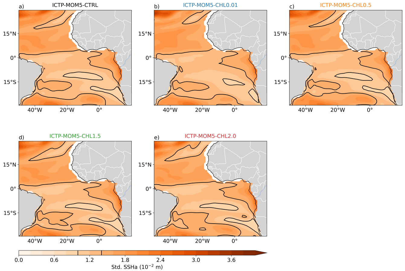
Figure A5. Standard deviation of detrended SSHa over the 1982-2020 for (a) ICTP-MOM5-CTRL, (b) ICTP-MOM5-CHL0.01, (c) ICTP-MOM5-CHL0.5, (d) ICTP-MOM5-CHL1.5, and (e) ICTP-MOM5-CHL2.0. Black contours denote the 0.01 m and 0.014 m standard deviation levels.
