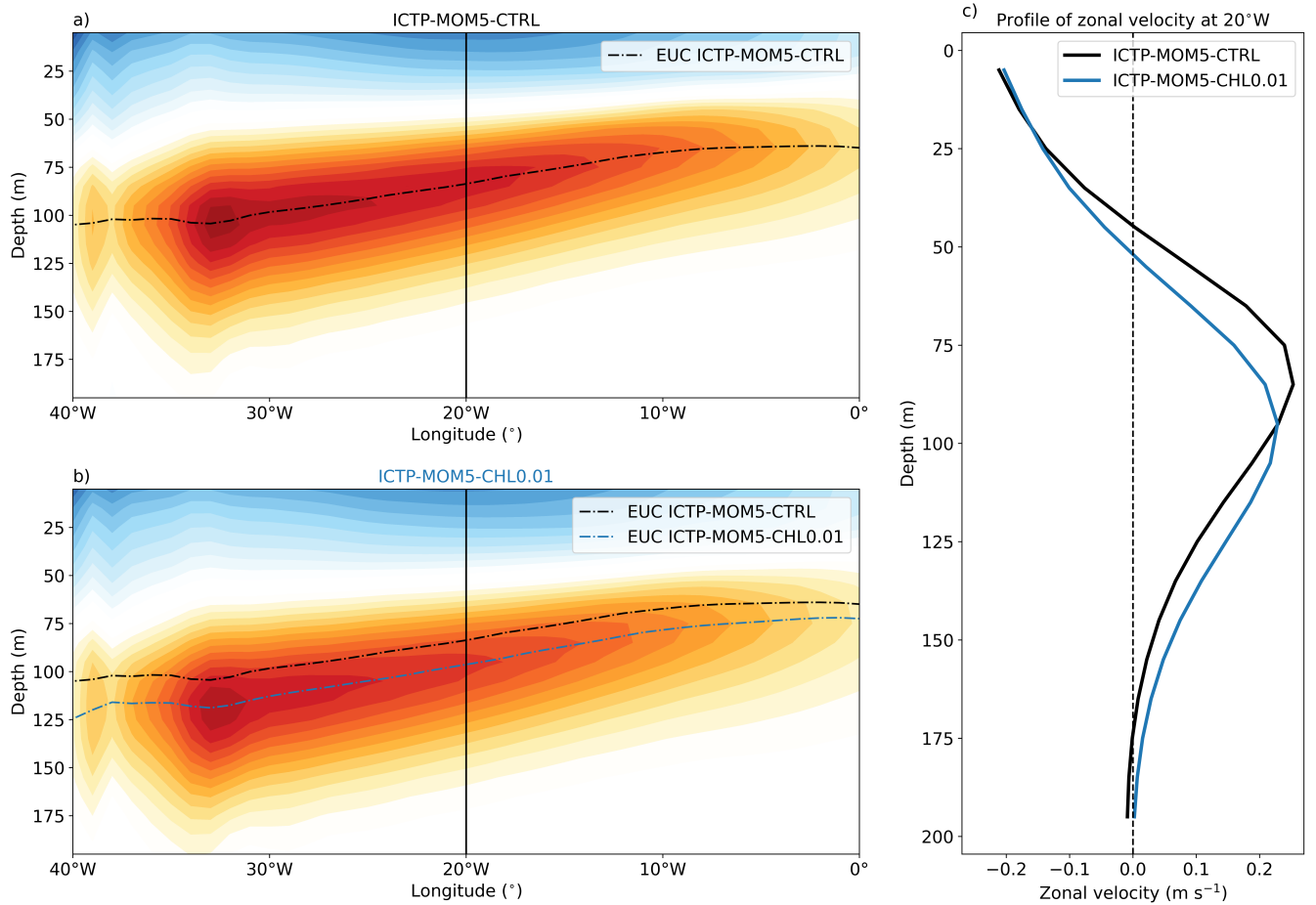
Figure A4. (a) Equatorial section (40°W-0°E; 3°S-3°N) of zonal velocity for (a) ICTP-MOM5-CTRL and (b) ICTP-MOM5-CH0.01 (blue). The dashed-dotted lines indicate the depth of the core of the equatorial undercurrent (EUC). The EUC depth is defined as the depth of the maximum eastward zonal velocity. For each vertical profile, the maximum velocity is first identified, and a quadratic interpolation through the maximum and its two neighboring depth levels is then used to estimate the peak depth continuously. If the maximum occurs at the upper or lower boundary, the corresponding model depth is retained. (c) Vertical profile of zonal velocity at 20°W, averaged between 3°S-°N, for ICTP-MOM5-CTRL (black) and ICTP-MOM5-CHL0.01 (blue).
