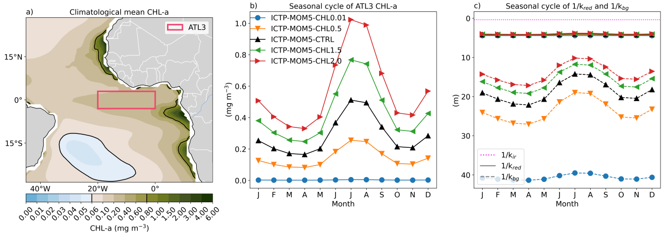
Figure 1. (a) Climatological mean chlorophyll-a concentration prescribed to ICTP-MOM5-CTRL. Black contours indicate the 0.06 \text{ mg m}^{-3} and 0.80 \text{ mg m}^{-3} chlorophyll-a concentration levels. (b) Seasonal cycle of the prescribed chlorophyll-a concentration averaged over the ATL3 ( 20^\circ\text{W} – 0^\circ\text{E} , 3^\circ\text{S} – 3^\circ\text{N} ) region and for the different model simulations: ICTP-MOM5-CHL0.01 (blue), ICTP-MOM5-CHL0.5 (orange), ICTP-MOM5-CTRL (black), ICTP-MOM5-CHL1.5 (green), and ICTP-MOM5-CHL2.0 (red). (c) Seasonal cycles of the e-folding depth scales of the light penetration in the ATL3 region for the infrared ( 1/k_{ir} , magenta dotted line), the red ( 1/k_{red} , full lines), and the blue/green ( 1/k_{bg} , dashed lines) wavelength bands. As 1/k_{red} and 1/k_{bg} depend on the chlorophyll-a concentration (cf. Eq. 2 and 3), the seasonal cycles are plotted for each model experiment.
