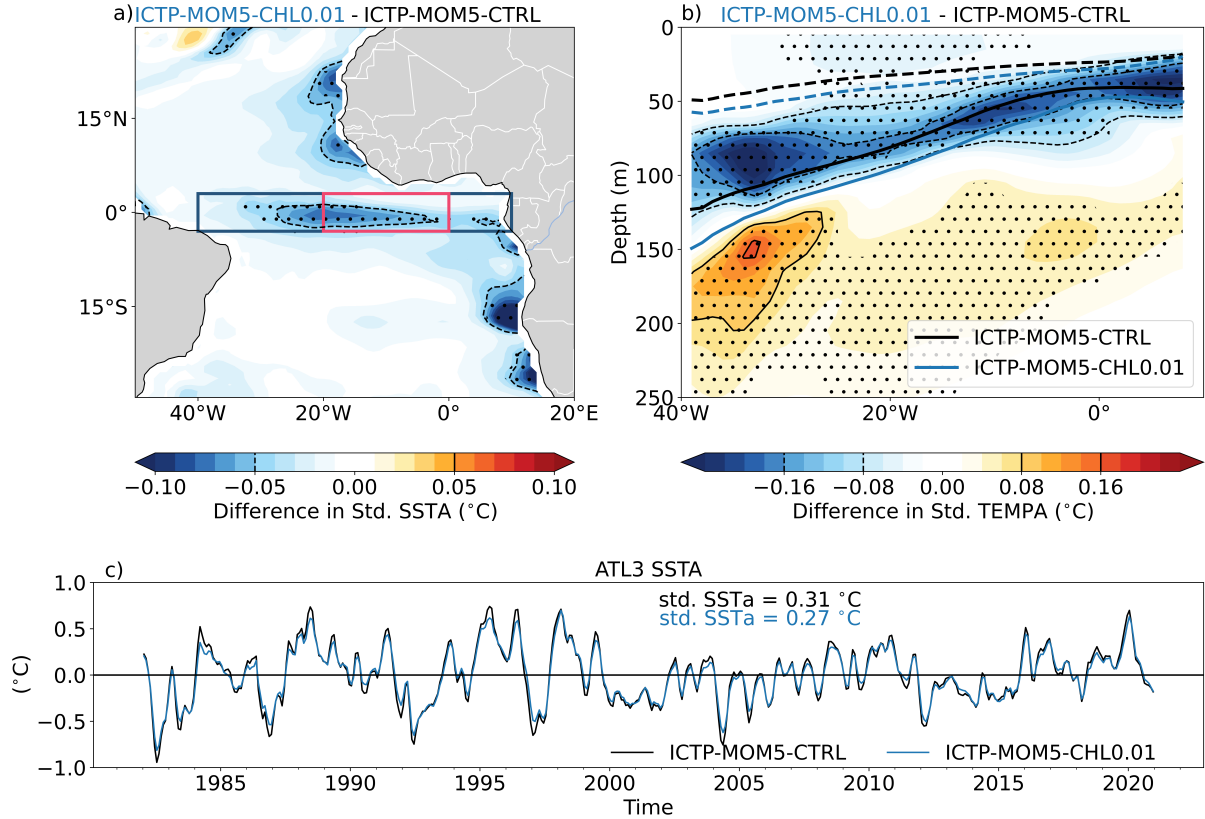
Figure 4. (a) Difference in the standard deviation of detrended SST anomalies between ICTP-MOM5-CHL0.01 and ICTP-MOM5-CTRL. Black dashed (solid) contours indicate -0.05 \text{ } ^\circ\text{C} ( 0.05 \text{ } ^\circ\text{C} ). The blue and red boxes denote the equatorial Atlantic (Eq. ATL; 40^\circ\text{W} – 10^\circ\text{E} , 3^\circ\text{S} – 3^\circ\text{N} ) and the ATL3 region ( 20^\circ\text{W} – 0^\circ\text{E} , 3^\circ\text{S} – 3^\circ\text{N} ) regions, respectively. (b) Difference in the standard deviation of the upper 250 m of the equatorial Atlantic TEMP anomalies between ICTP-MOM5-CHL0.01 and ICTP-MOM5-CTRL. Black dashed (solid) contours indicate -0.16 \text{ } ^\circ\text{C} and -0.08 \text{ } ^\circ\text{C} ( 0.08 \text{ } ^\circ\text{C} and 0.16 \text{ } ^\circ\text{C} ). Black stipplings in (a) and (b) indicate regions where the difference in standard deviation is statistically significant at the 99% level according to a bootstrap test (see Sect. 2.3). (c) Time series of detrended ATL3-averaged SST anomalies for ICTP-MOM5-CTRL (black) and ICTP-MOM5-CHL0.01 (blue).
