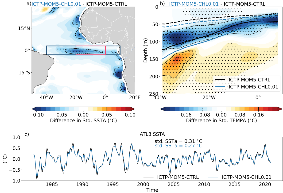
Figure 4. (a) Difference in the standard deviation of detrended SST anomalies between ICTP-MOM5-CHL0.01 and ICTP-MOM5-CTRL. Black dashed (solid) contours indicate -0.05 – -0.05 °C (0.05 °C). The blue and red boxes denote the equatorial Atlantic (Eq. ATL; 40°W–10°W–10°E, 3°S–3°S–3°N) and the ATL3 region (20°W–0°W–0°E, 3°S–3°S–3°N) regions, respectively. (b) Difference in the standard deviation of the upper 250 m of the equatorial Atlantic TEMP anomalies between ICTP-MOM5-CHL0.01 and ICTP-MOM5-CTRL. Black dashed (solid) contours indicate -0.16 – -0.16 °C and -0.08 – -0.08 °C (0.08 °C and 0.16 °C). Black stipplings in (a) and (b) indicate regions where the difference in standard deviation is statistically significant at the 99% level according to a bootstrap test (see Sect. 2.3). (c) Time series of detrended ATL3-averaged SST anomalies for ICTP-MOM5-CTRL (black) and ICTP-MOM5-CHL0.01 (blue).
