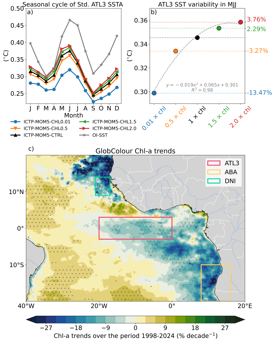
Figure 5. (a) Seasonal cycle of the standard deviation of the detrended SSTA-SST anomalies averaged over the ATL3 region for ICTP-MOM5-CHL0.01 (blue), ICTP-MOM5-CHL0.5 (orange), ICTP-MOM5-CTRL (black), ICTP-MOM5-CHL1.5 (green) and ICTP-MOM5-CHL2.0 (red). The red, orange, and green boxes indicate the ATL3, ABA (8°E-16°E, 20°S-10°S), and DNI (21°W-17°W, 9°N-14°N) regions, respectively. (b) Scatter diagrams showing the standard deviation of SSTAs-SST anomalies averaged over the ATL3 region in function of the prescribed Chl-a seasonal cycle as indicated on the x-axes. The right y-axis shows the percentage of change in SST variability relative to the ICTP-MOM5-CTRL value. (c) Linear trends in Chl-a over January 1998-December 2024. Trends are computed from a linear least-squares fit applied to monthly mean Chl-a time series at each grid point. The trend-resulting slope (mg m -3 month -1 ) is converted to mg m -3 decade -1 by multiplying by 120 (12 months × 10 years). Relative trends are then expressed in % decade -1 and calculated from the linear slope evaluated using monthly means of the daily gap-free product, then multiplied by 120, divided dividing by the climatological mean chlorophyll concentration at each grid point, and multiplied multiplying by 100. Grey stipplings indicate regions showing a statistically significant trend at the 95% level according to a Student's t-test.
