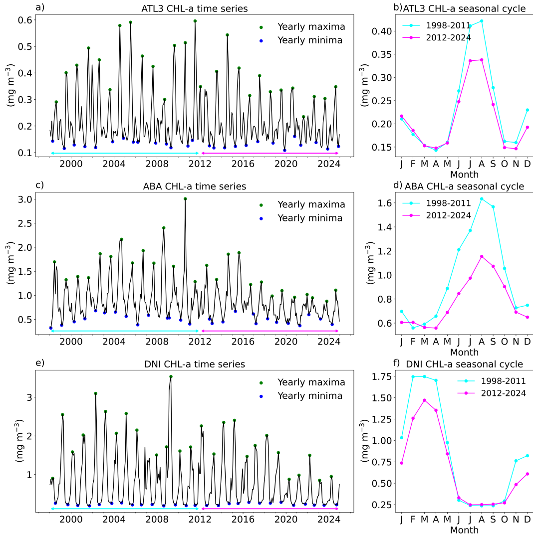
Figure 6. (a) Time series of chlorophyll-a concentration Chl-a from the GlobColour satellite ocean colour product , averaged over the ATL3 region, for the period from 1998/01 to 2024/12. Green (blue) dots indicate the yearly maxima (minima). The cyan (magenta) arrow denotes the period from 1998/01-2011/12 (2012/01-2024/12). (b) Seasonal cycle of the ATL3 chlorophyll-a Chl-a from GlobColour evaluated over 1998-2011 (cyan) and 2012-2024 (magenta). (c, d) Same as (a, b) but for the ABA (orange box in Fig. 5c; 8°E-16°E, 20°S-10°S) region. (e, f) Same (a, b) but for the DNI (green box in Fig. 5c; 21°W-17°W, 9°N-14°N) region.
