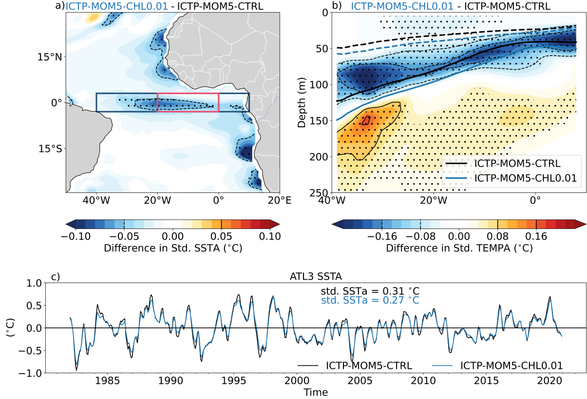
Figure 4. (a) Difference in the standard deviation of detrended SSTA-SST anomalies between ICTP-MOM5-CHL0.01 and ICTP-MOM5-CTRL. Black dashed (solid) contours indicate -0.05^{\circ}\text{C} ( 0.05^{\circ}\text{C} ). The blue and red boxes denote the equatorial Atlantic (Eq. ATL; 40^{\circ}\text{W} – 10^{\circ}\text{E} , 3^{\circ}\text{S} – 3^{\circ}\text{N} ) and the ATL3 region ( 20^{\circ}\text{W} – 0^{\circ}\text{E} , 3^{\circ}\text{S} – 3^{\circ}\text{N} ) regions, respectively. (b) Difference in the standard deviation of the upper 250 m of the equatorial Atlantic TEMPA-TEMP anomalies between ICTP-MOM5-CHL0.01 and ICTP-MOM5-CTRL. Black dashed (solid) contours indicate -0.16^{\circ}\text{C} and -0.08^{\circ}\text{C} ( 0.08^{\circ}\text{C} and 0.16^{\circ}\text{C} ). Black stipplings in (a) and (b) indicate regions where the difference in standard deviation is statistically significant at the 99% level according to a bootstrap test (see Sect. 2.3.1). (c) Time series of detrended ATL3-averaged SSTA-SST anomalies for ICTP-MOM5-CTRL (black) and ICTP-MOM5-CHL0.01 (blue).
