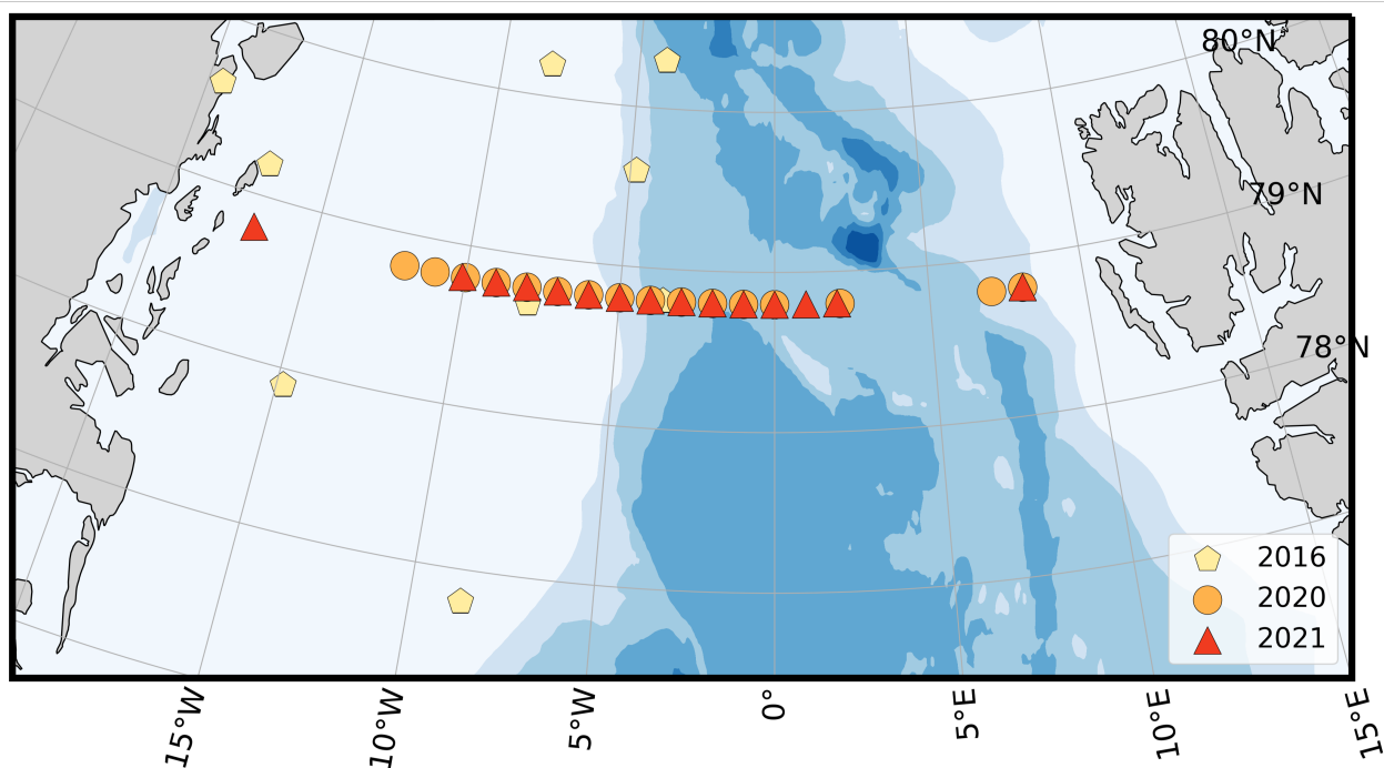
Figure A2. Overview map of all stations in 2016, 2020, and 2021. The data from 2016 is taken from Wefing et al. (2019) Wefing et al. (2019) .
