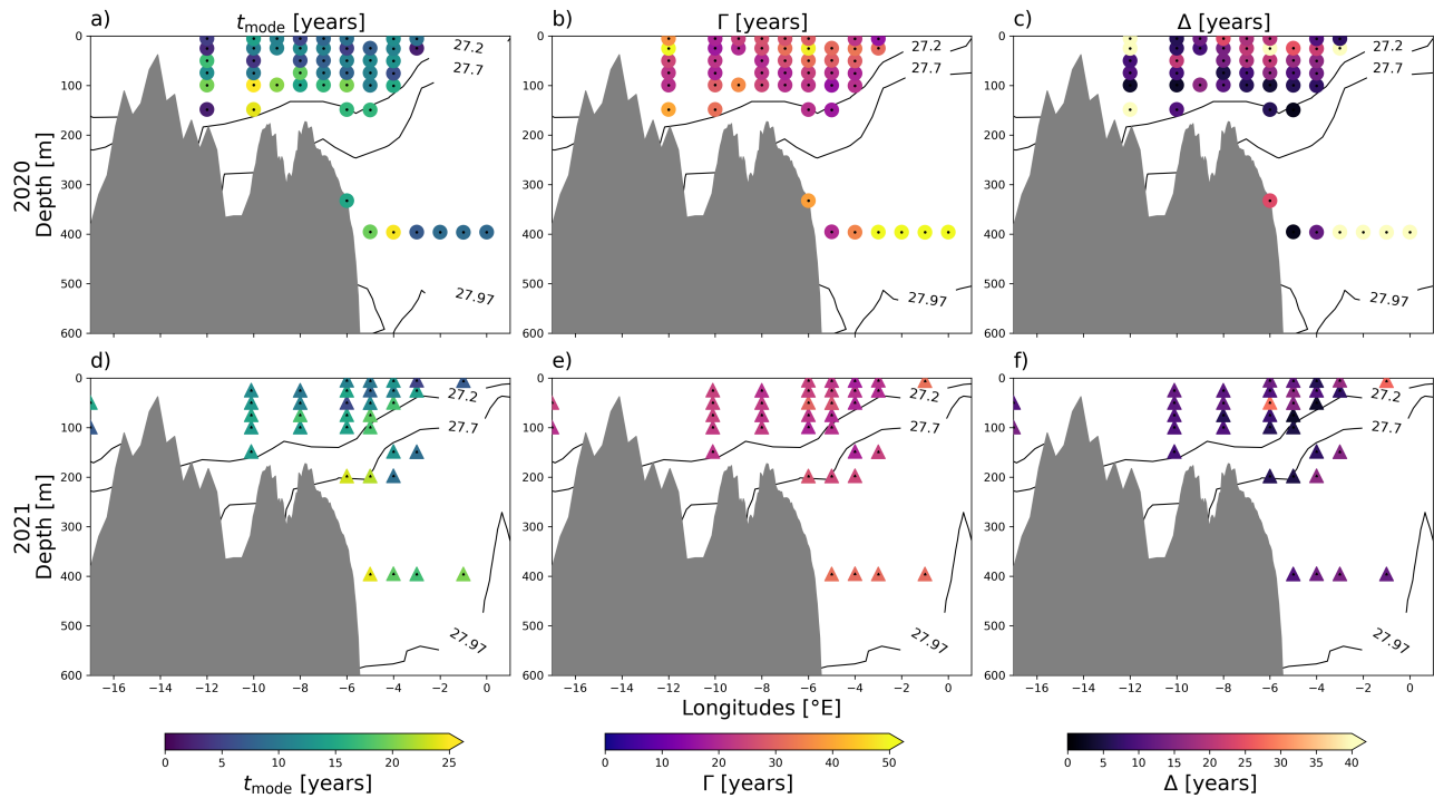
Figure A7. TTD parameters t_{mode} (a,d), \Gamma (b,e), and \Delta (c,f) for 2020 (a,b,c) and 2021 (d,e,f). Results are shown for Polar Water I and Arctic Atlantic Water. Selected \sigma_0 isopycnals (black) for \sigma_0 = (27.2, 27.7, 27.97) are overlaid.
