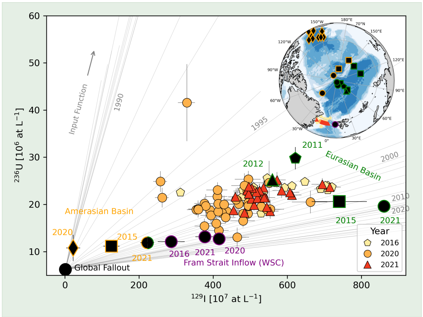
Figure 9. Polar Water I samples from 2016 (yellow), 2020 (blueorange), and 2021 (red) are displayed in the ^{129}\text{I} against ^{236}\text{U} tracer space. Previous measurements with the same densities as Polar Water I from 2011, 2012, 2015, 2020, and 2021 are shown as yearly averaged concentrations separately for Amerasian and Eurasian stations. Amerasian-origin waters (orange outline, station locations indicated in the inset map ) are represented by samples taken from the Canadian and Makarov Basins, sampled during different expeditions in 2015 (stations 96, 101, and 134 from Casacuberta et al. (2018) Casacuberta et al. (2018) , squares), 2020 (all stations from Payne et al. (2024) Payne et al. (2024) , diamonds), and 2021 (stations 28 and 46 from Wefing et al. (2025) Wefing et al. (2025) , circles). Eurasian-origin waters (green outline, station locations indicated in the inset map ) are represented by stations in the Amundsen and Nansen Basins, sampled in 2011 (station 212 from Casacuberta et al. (2016) Casacuberta et al. (2016) , pentagon), 2012 (station 378 from Casacuberta et al. (2016) Casacuberta et al. (2016) , triangle), 2015 (stations 68, 81, 117, and 125 from Casacuberta et al. (2018) Casacuberta et al. (2018) , squares), and 2021 (stations 16 and 20 from Wefing et al. (2025) Wefing et al. (2025) , circles). The global fallout tracer signature is indicated as a black circle ( 1.16 \times 10^7 at \text{L}^{-1} for ^{129}\text{I} and 6.25 \times 10^6 at \text{L}^{-1} for ^{236}\text{U} ( Snyder et al., 2010 ; Chamizo et al., 2022 ) ( Snyder et al., 2010 ; Chamizo et al., 2022 )). Incoming WSC waters (purple outline) are represented as averaged tracer signatures of the upper 100 m at 7^\circ \text{E} / 8^\circ \text{E} in 2016, 2020, and 2021. The surface NCC input function is shown as grey lines with some specific years for orientation. The inset map shows the geographical location of the samples and upstream tracer signatures.
