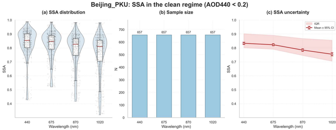
Figure 5: SSA statistics in the clean regime (AOD440 < 0.2) at Beijing_PKU. Panel (a) shows the SSA distribution at four wavelengths, where the violin shape indicates kernel density, the box indicates the median and interquartile range, and the gray dots denote individual samples. Panel (b) shows the sample size at each wavelength. Panel (c) shows the wavelength-dependent SSA mean, 95% bootstrap confidence interval, and interquartile range.
