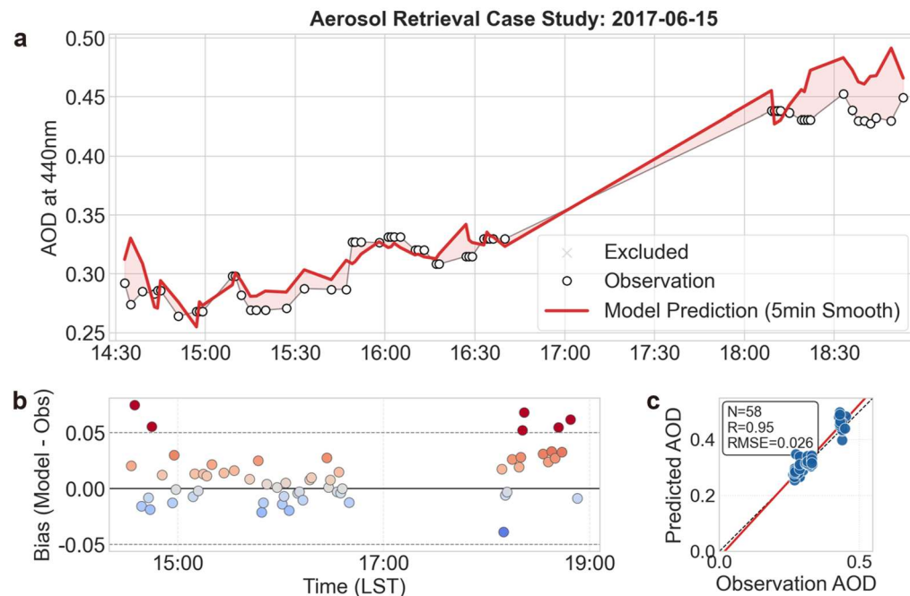
Figure 96: Case study of diurnal AOD variation retrieval at the Beijing site on June 15, 2017. The top panel (a) compares the AERONET observations (black circles) with the model predictions that have not been independently validated (red solid line, smoothed using a 5-minute time window). The bottom panels display the time series of retrieval bias (b) and the scatter plot between observed and predicted AOD (c). For visualization only, a 5-minute moving average was applied to the ASI retrievals in Fig. 9a to reduce point-to-point noise and highlight the overall diurnal trend. All statistical metrics reported in this study, however, were calculated from the original unsmoothed retrievals.
