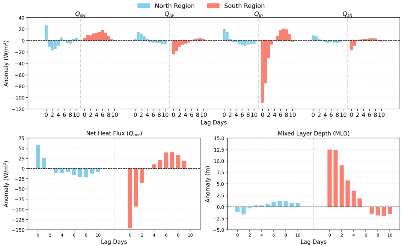
Figure 9. Composite anomalies (strong minus weak dust events) of surface heat flux components ( \text{W/m}^2 ), net surface heat flux ( Q_{\text{net}} , \text{W/m}^2 ), and MLD (m) over the northern (blue) and southern (red) regions. All flux components are defined as positive downward (into the ocean). The upper panel shows anomalies of net shortwave radiation ( Q_{\text{sw}} ), net longwave radiation ( Q_{\text{lw}} ), latent heat flux ( Q_{\text{lh}} ), and sensible heat flux ( Q_{\text{sh}} ). The lower-left panel presents anomalies in Q_{\text{net}} , and the lower-right panel shows the corresponding anomalies in MLD. The x-axis represents lag days (0–10) relative to dust onset.
