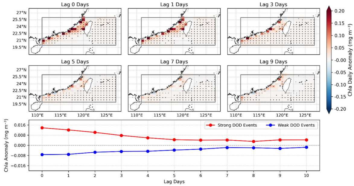
Figure 4. Same as Figure 3, but for Southern Region.
