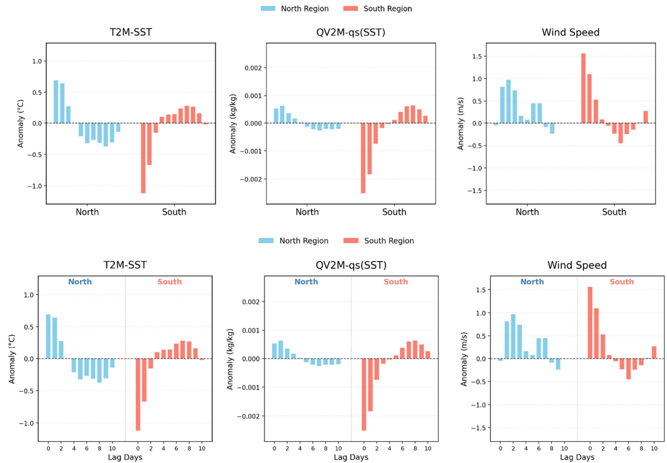
Figure 8. Composite anomalies of air–sea temperature difference (left; T2M–SST), air–sea specific humidity difference (middle; QV2M– q_s (SST)), and surface wind speed (right) associated with strong minus weak dust events over the northern (blue) and southern (red) regions. The horizontal axis shows lag days from lag 0 (dust-onset) to lag 10.
