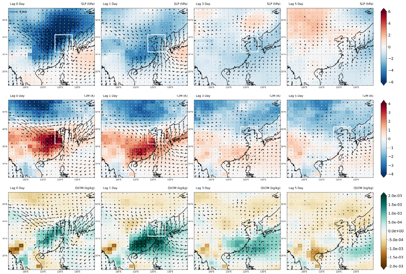
Figure 6. Composite anomalies (strong minus weak dust events) of atmospheric circulation fields for the Northern Region at lag 0, 1, 3, and 5 days relative to dust event onset. Rows show (top) sea level pressure (SLP, hPa), (middle) 2 m air temperature (T2M, K), and (bottom) 2 m specific humidity (QV2M, kg kg -1 ). Anomalous 10 m wind vectors (m s -1 ) are overlaid on all panels. The white box denotes the Northern Region. Stippling denotes areas where anomalies are statistically significant at the 95% confidence level ( p < 0.05 ).
