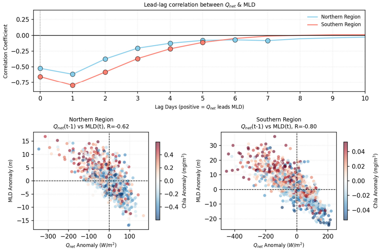
Figure 10. Lead-lag relationship between Q_{net} and MLD anomalies during spring over the 2003-2023 period. The upper panel shows the lead-lag correlation coefficients for the northern (blue) and southern (red) regions, where positive lag indicates that Q_{net} leads MLD. Horizontal dashed lines denote the 99.9% significance level, and the vertical grey line marks zero lag. Filled circles denote correlations that are statistically significant at the 95% confidence level ( p < 0.05 ), and the vertical grey line marks zero lag. The lower panels show scatterplots of Q_{net} anomalies at day t-1 versus MLD anomalies at day t for the Northern (left) and Southern (right) regions. Marker colors indicate the concurrent Chl- a anomaly at day t .
