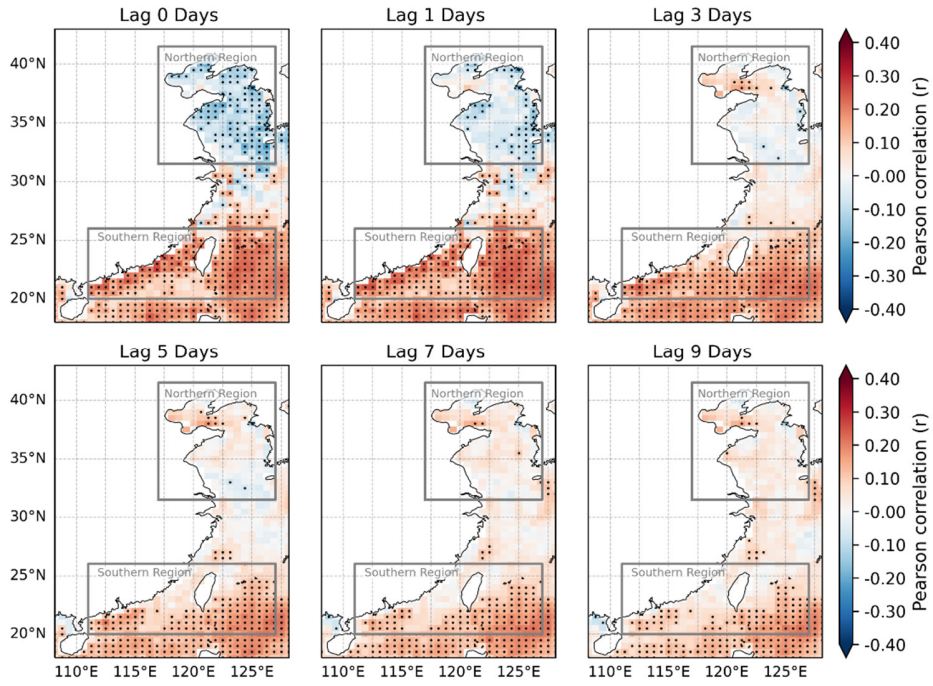
Figure 2. Spatial distributions of lagged Pearson correlation coefficients between dust optical depth (DOD) and chlorophyll-a (Chl-a) concentration along China's coastal seas. Correlations are calculated with dust leading Chl-a by 0, 1, 3, 5, 7, and 9 days. Stippling indicates correlations significant at the 95% confidence level ( p < 0.05 ). Dark gray boxes denote the Northern Region (117–127°E, 31.5–41.5°N) and the Southern Region (111–127°E, 20–26°N).
