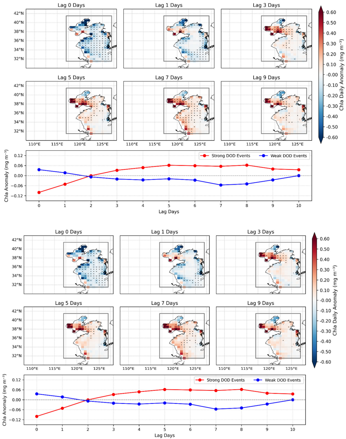
Figure 3. Composite analysis of chlorophyll-a (Chl- a ) responses to extreme dust events in the Northern Region (31.5°–41.5°N, 117°–127°E). The upper panels show the spatial distribution of the differences in Chl- a daily anomalies between strong (>95th percentile) and weak (<5th percentile) dust events at lags of 0, 1, 3, 5, 7, and 9 days, with DOD leading and Chl- a lagging. Stippling denotes grid points where the differences are statistically significant at the 95% confidence level ( p < 0.05 ). The lower panel illustrates the temporal evolution of regionally averaged Chl- a daily anomalies for strong (red) and weak (blue) dust events as a function of lag days.
