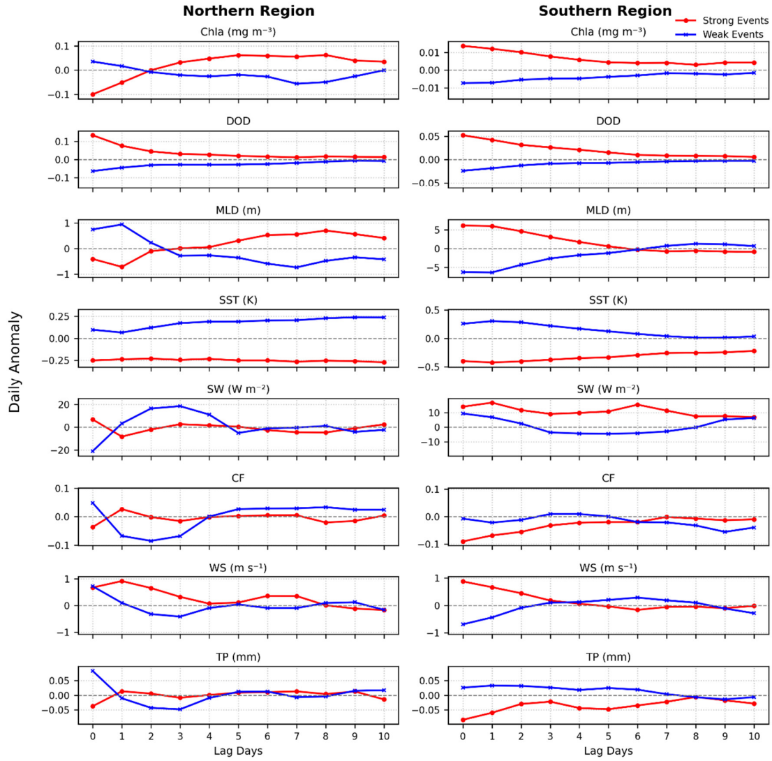
Figure 5. Composite temporal evolution of daily anomalies in chlorophyll-a ( \text{Chl-a} , \text{mg m}^{-3} ), dust optical depth ( DOD ), mixed layer depth (MLD, m), sea surface temperature (SST, K), shortwave radiation (SW, \text{W m}^{-2} ), cloud fraction (CF), wind speed (WS, \text{m s}^{-1} ), and total precipitation (TP, mm) for the Northern Region (left column) and Southern Region (right column). Red lines with filled circles denote strong dust events (>95th percentile); blue lines with crosses denote weak dust events (<5th percentile). The horizontal axis indicates lag days relative to dust event onset (lag 0). The gray dashed line marks the zero-anomaly reference. Only oceanic grid points within each region are included.
