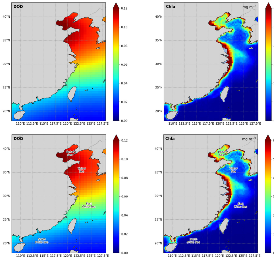
Figure 1. Spring climatological mean distributions of (left) DOD dust-optical-depth and (right) Chlorophyll-a-a concentration (unit: \text{mg/m}^3 ) over the Chinese marginal seas, averaged over 2003–2023.
