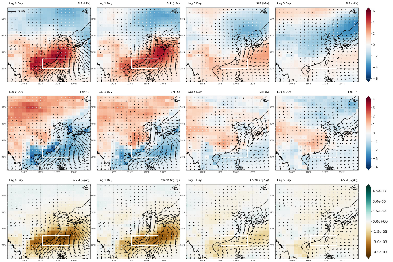
Figure 7. Same as Figure 6, but for Southern Region (indicated in the white box).
