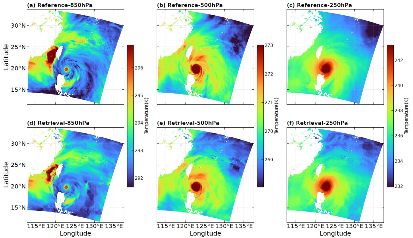
430 Figure 9. Spatial distributions of the simulated temperature fields by the WRF model (upper row), and retrieved temperature fields (bottom row) at different pressure levels (from left to right: 850 hPa, 500 hPa, and 250 hPa) for the Typhoon Doksuri case at 25 July 2023.
