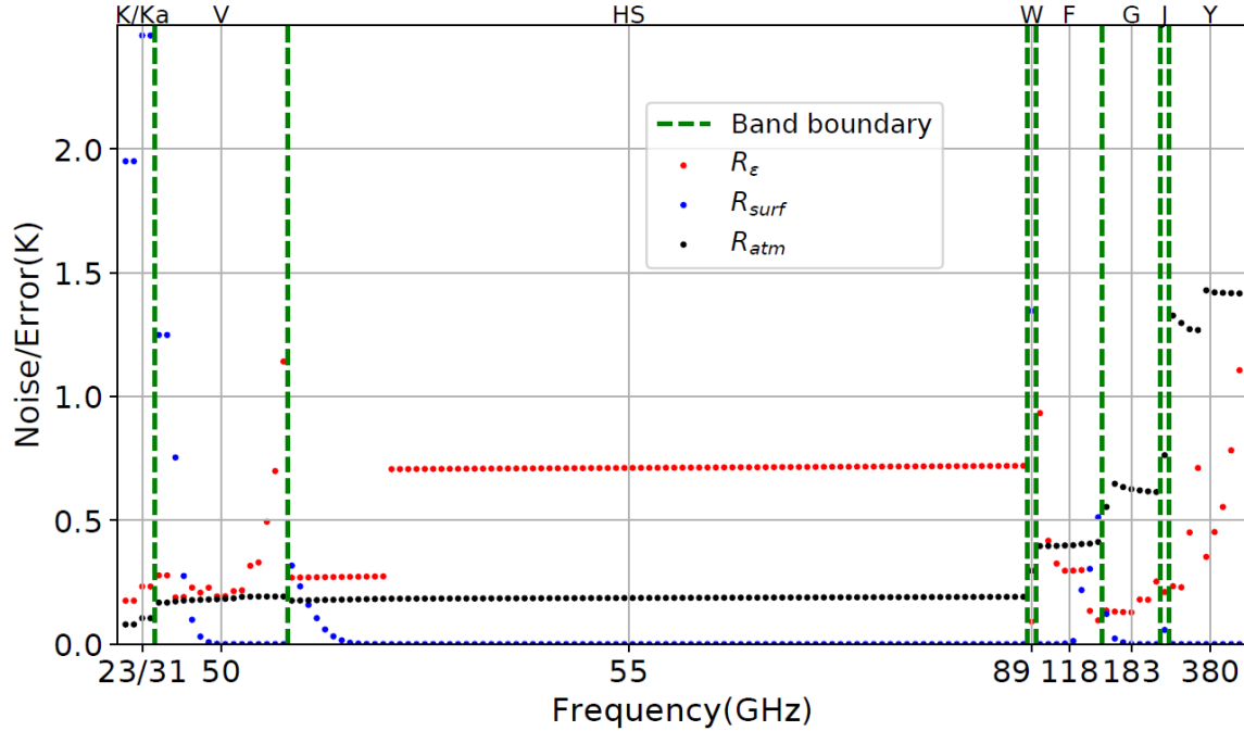
Figure 2. Instrument noise R_\varepsilon and radiative transfer errors induced by the atmosphere ( R_{atm} ) and surface ( R_{surf} ) for various channels of the FY-4M satellite. Green dashed lines indicate band boundaries.
