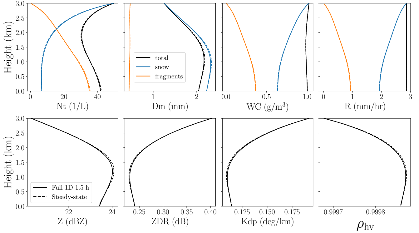
Figure 10. Moments and forward simulated radar variable comparison of a full time and height snow aggregation/breakup BinMod1D model run at t = 1.5 h compared to the corresponding steady-state BinMod1D model run.
