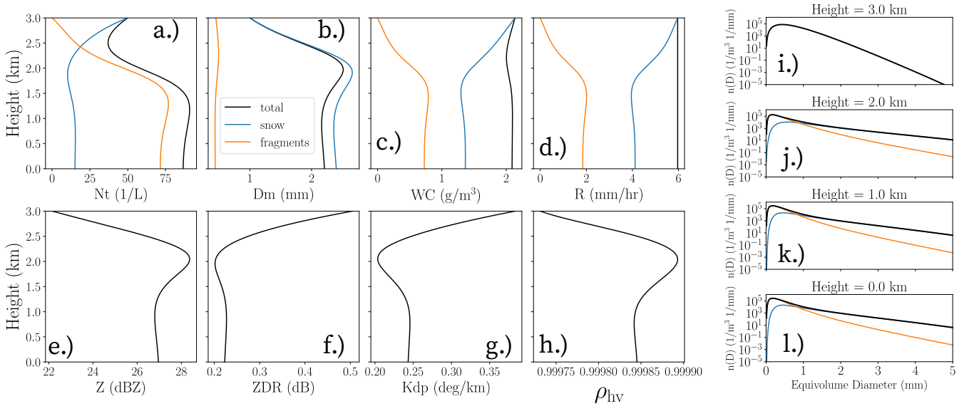
Figure 7. As in Figure 6 but for snow aggregation and collisional breakup as described in text. Here, s_{\text{bin}} = 3 and \Delta z = 5 m.
