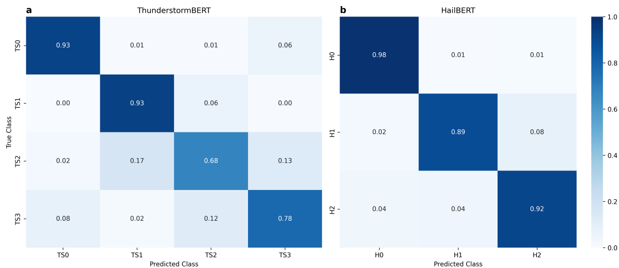
Figure 15. Normalised confusion matrix for ThunderstormBERT and HailBERT on the independent held-out test dataset. For each true class (row), the probability that the model will predict this class correctly (diagonally) or as a different class is shown.
