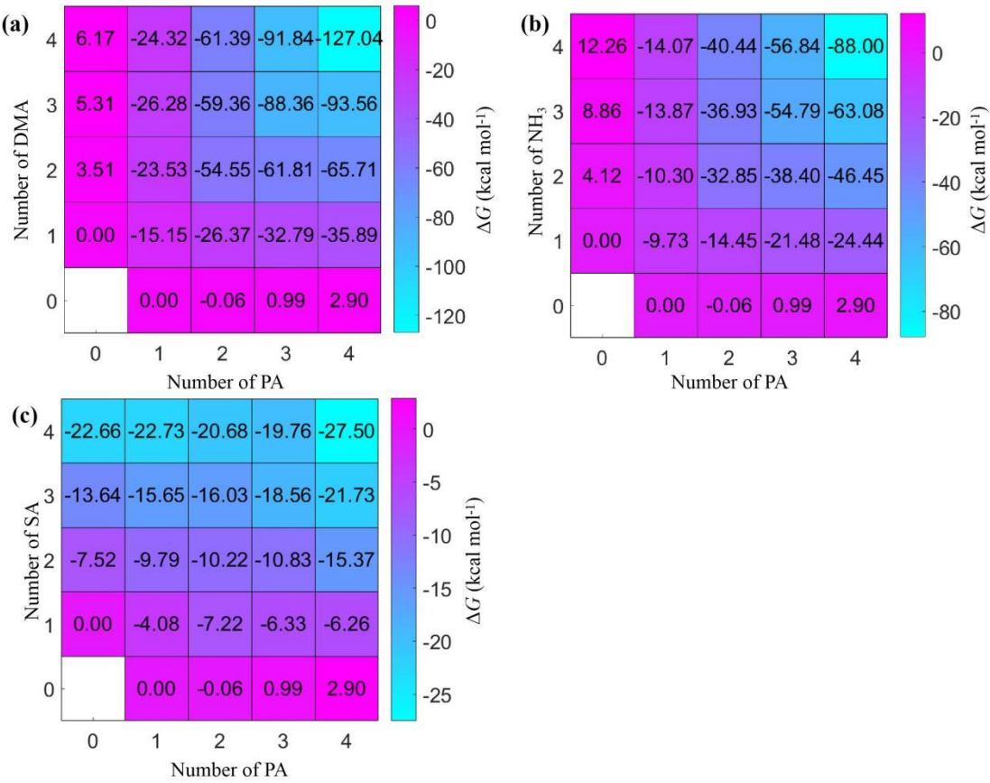
536 Figure 2. At the DLPNO-CCSD(T)/aug-cc-pVTZ// \omega B97X-D/6-31++G(d,p) level of 537 theory, the formation free energy ( \Delta G ) (in kcal mol -1 ) of (a) (PA) 1-4 (DMA) 1-4 , (b) 538 (PA) 1-4 (NH 3 ) 1-4 and (c) (PA) 1-4 (SA) 1-4 clusters. The computations are carried out at 1 539 atm and 278 K.
