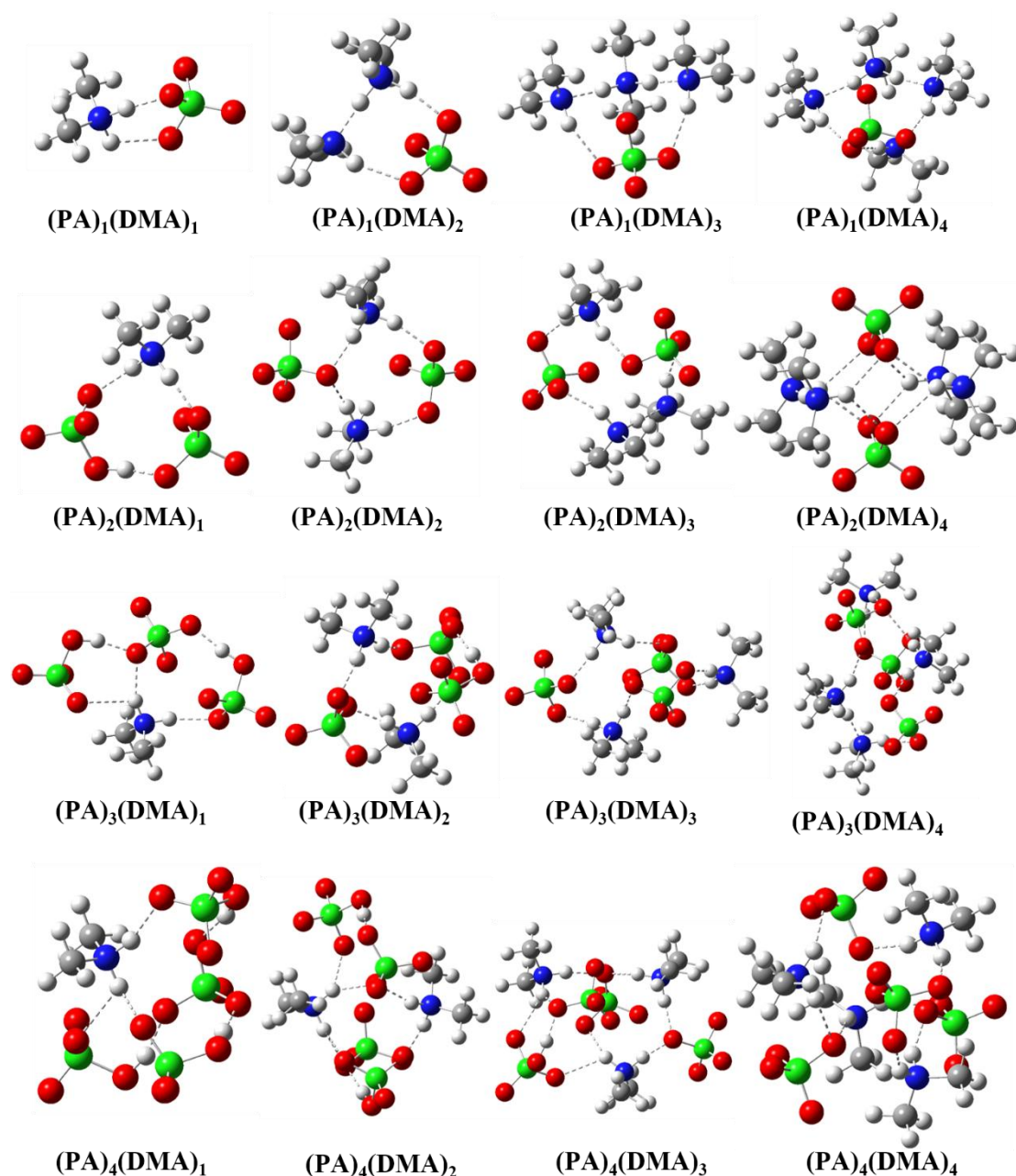
Figure 1. Identified minimum free energy configurations of the (\text{PA})_{1-4}(\text{DMA})_{1-4} clusters at the DLPNO-CCSD(T)/aug-cc-pVTZ// \omega B97X-D/6-31++G(d,p) level of theory. The atoms of oxygen, nitrogen, chlorine, carbon, and hydrogen are represented by the red, blue, green, gray, and white balls, respectively. Hydrogen bonds are indicated by the dashed white lines.
