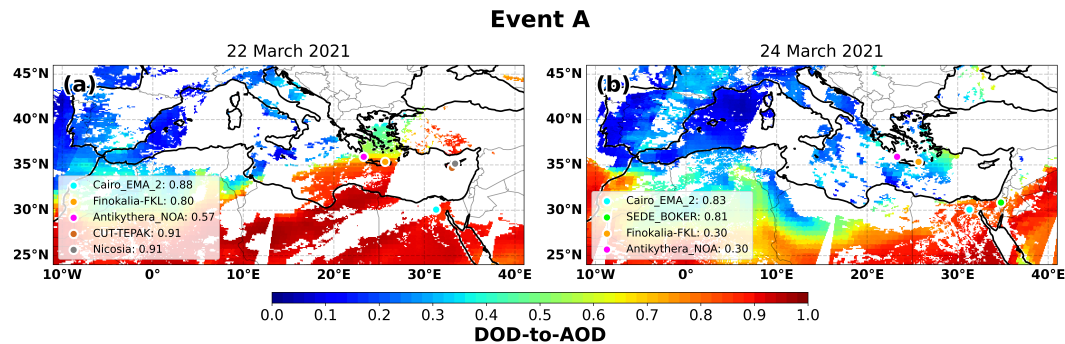
Figure C1. DOD-to-AOD ratios (at 550 nm) over the Mediterranean Basin from MIDAS for event A. The days with the available almucantar AERONET retrievals are displayed along with the specific stations (colored circles).
