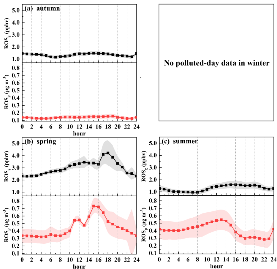
Figure 8. Seasonal diurnal profiles of ROS_g and ROS_p on polluted days
