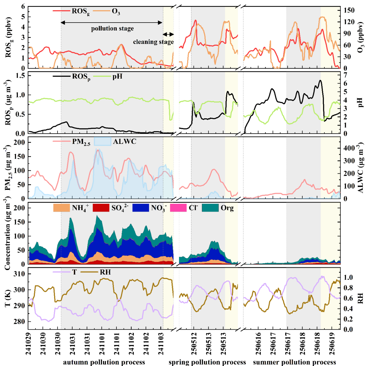
570 Figure 10. Typical pollution processes observed in different seasons
