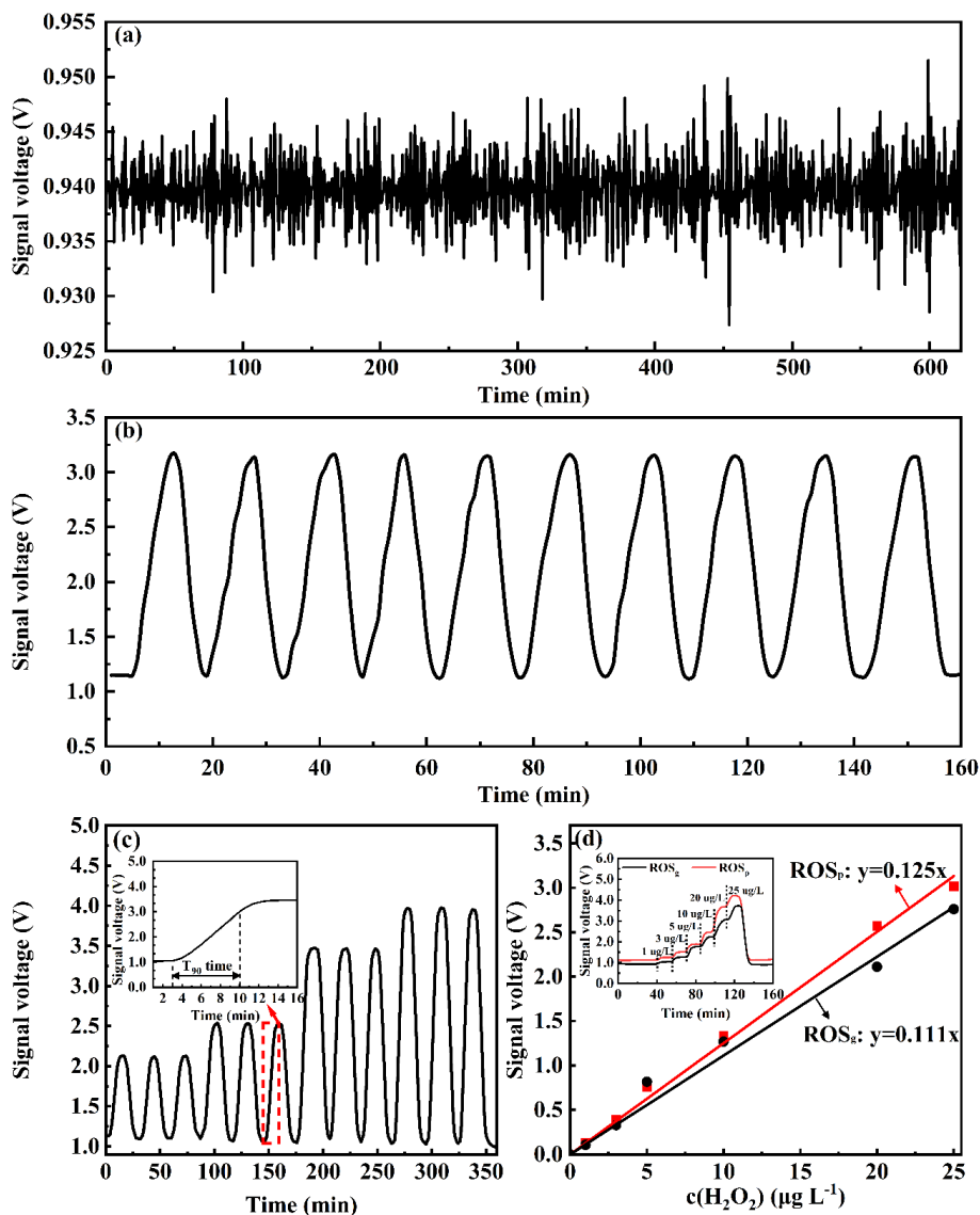
310 Figure 3. Performance evaluation of the atmospheric ROS online analyzer: (a) baseline stability, (b) reproducibility, (c) sensitivity, and (d) linear working range.
