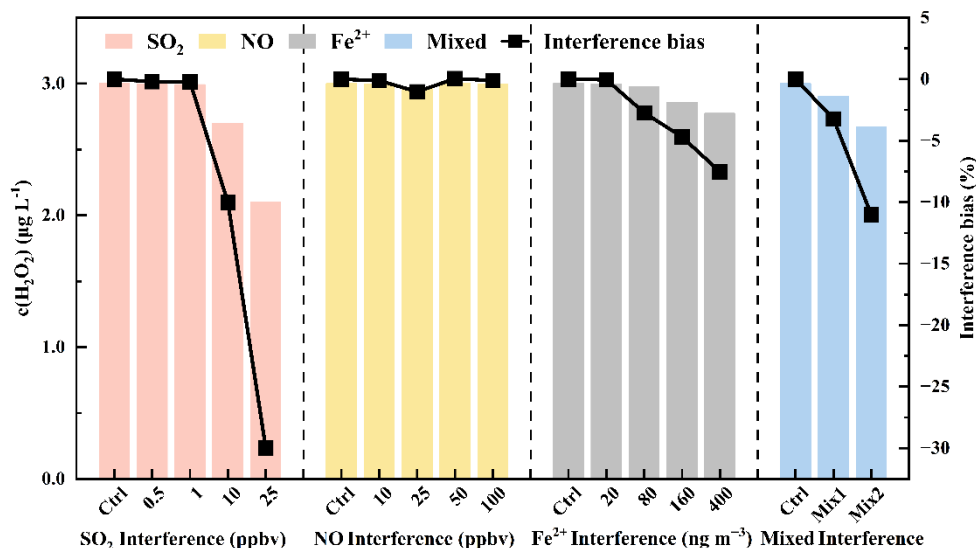
Figure 4. Effects of SO 2 , NO, Fe 2+ , and mixed interferents on the DCFH-HRP response to 3 μg L −1 H 2 O 2 . SO 2 and NO levels are given in ppbv, and Fe 2+ levels in ng m −3 . Mix1 contains 1 ppbv SO 2 , 25 ppbv NO, and 80 ng m −3 Fe 2+ , while Mix2 contains 10 ppbv SO 2 , 100 ppbv NO, and 160 ng m −3 Fe 2+ . Bars indicate measured H 2 O 2 -equivalent concentrations, and black squares indicate interference bias relative to the control.
