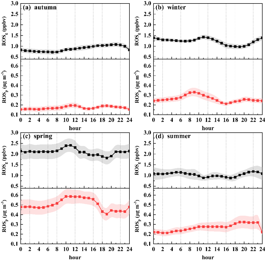
Figure 7. Seasonal diurnal profiles of \text{ROS}_g and \text{ROS}_p on clean days
